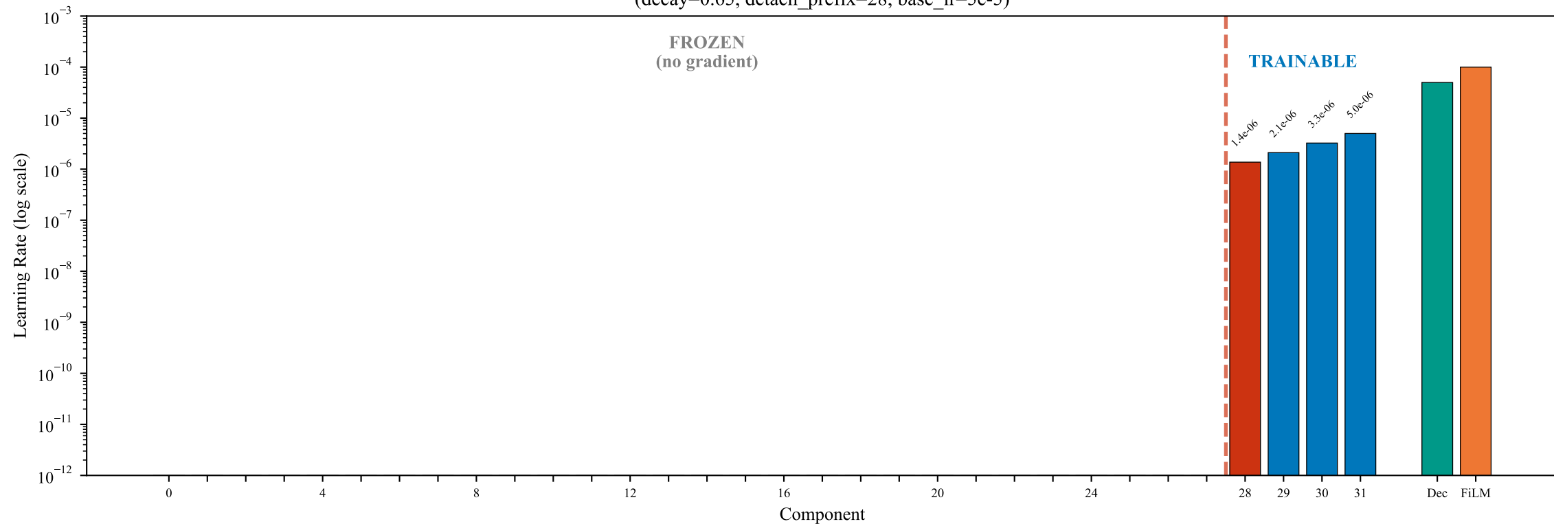
LLRD + Detach Prefix Learning Rate Assignment (decay=0.65, detach_prefix=28, base_lr=5e-5)
