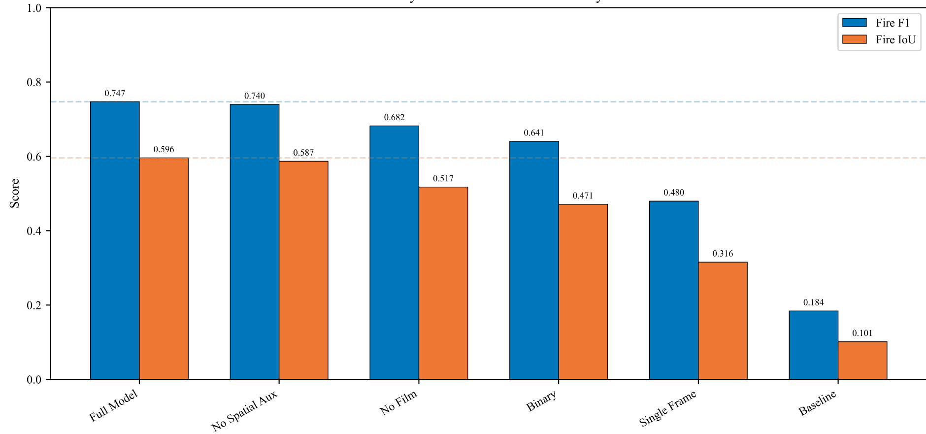
Ablation Study: Fire Detection Performance by Variant
