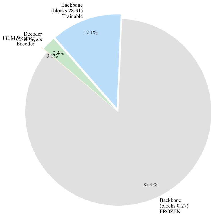
(a) Total Parameters: 646.8M
