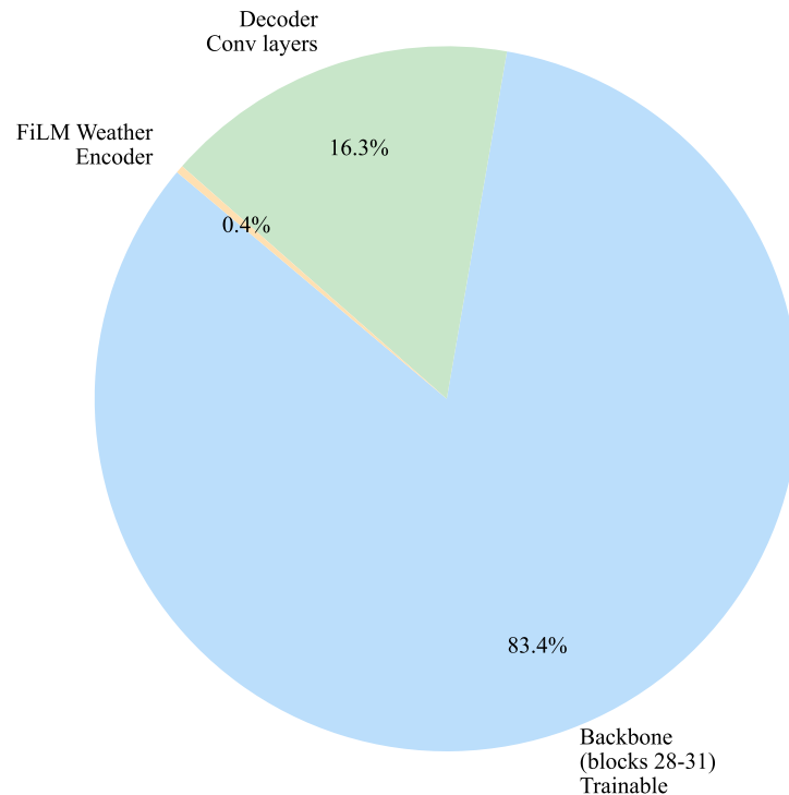
(b) Trainable Parameters: 94.1M (14.5%)
