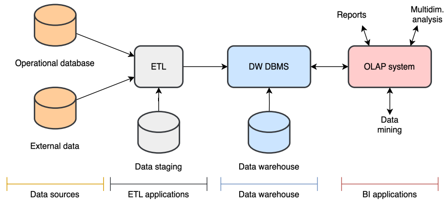
Figure 1.3: Three-Layer Architecture.
