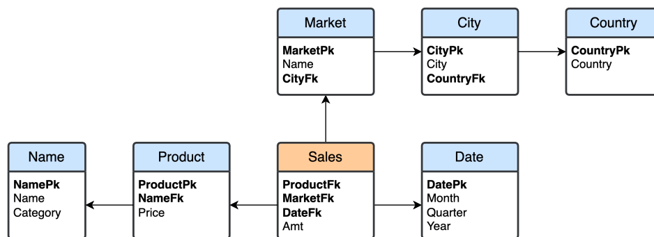
Figure 2.8: Example of a snowflake schema.
