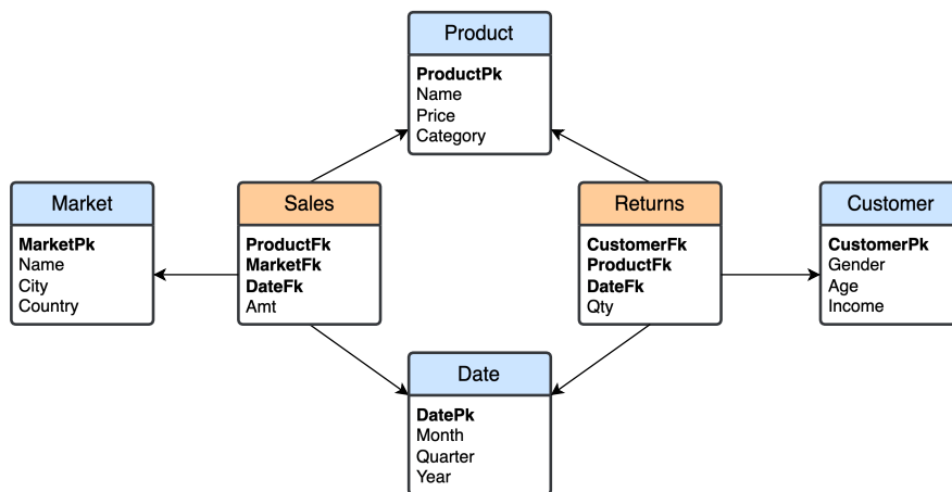
Figure 2.9: Example of a constellation schema.
