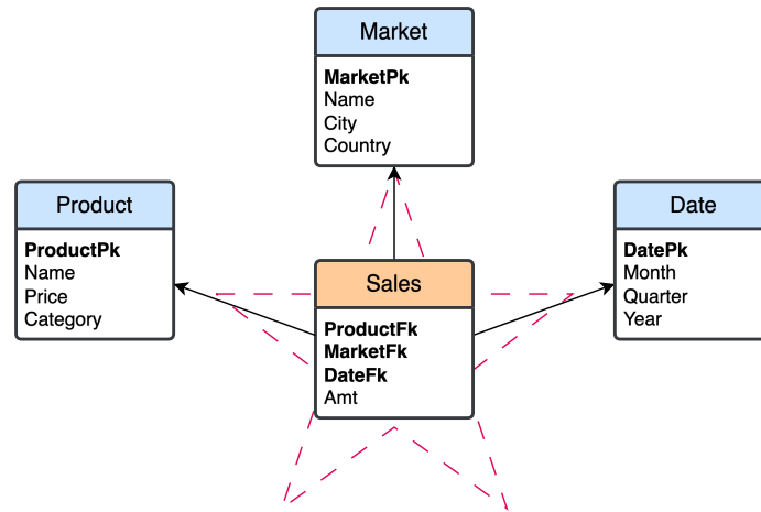
Figure 2.7: Example of a star schema.
