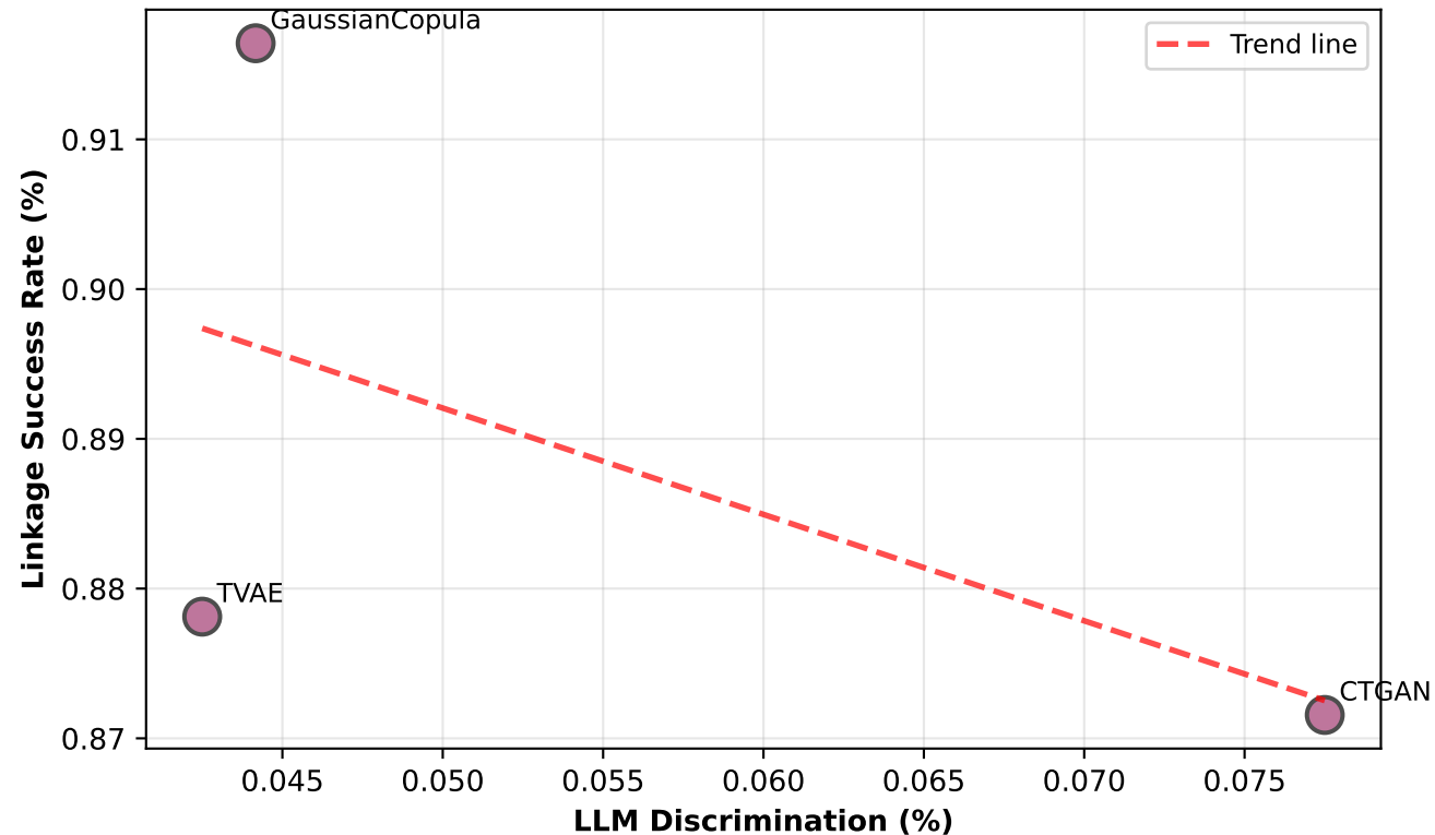
LLM vs Linkage Risk r = -0.5788 ( p = 0.6070 )
