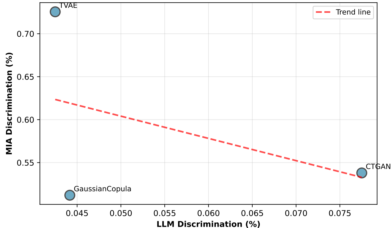
LLM vs MIA r = -0.4388 ( p = 0.7108 )
