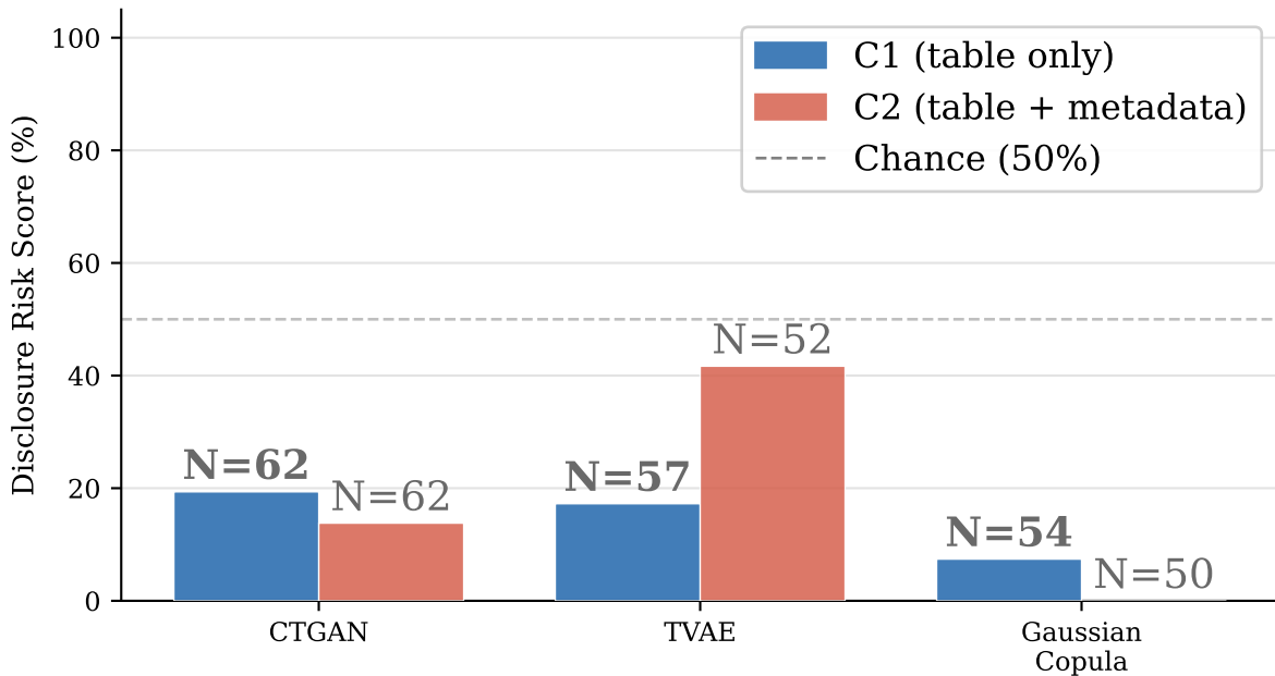
Adult Dataset — Disclosure Risk Score by Method & Condition (N=337 valid trials, approved providers)
