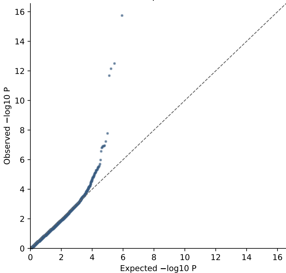
Interaction Q-Q plot ( \lambda_{GC} = 0.929 )
