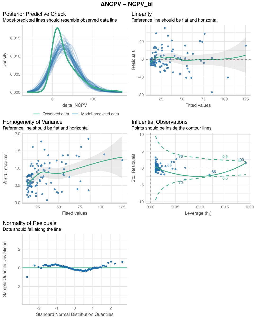
Figure 1: performance::check_model(lm( \Delta\text{NCPV} \sim \text{NCPV}_{bl} )) output for the reported change-score model
