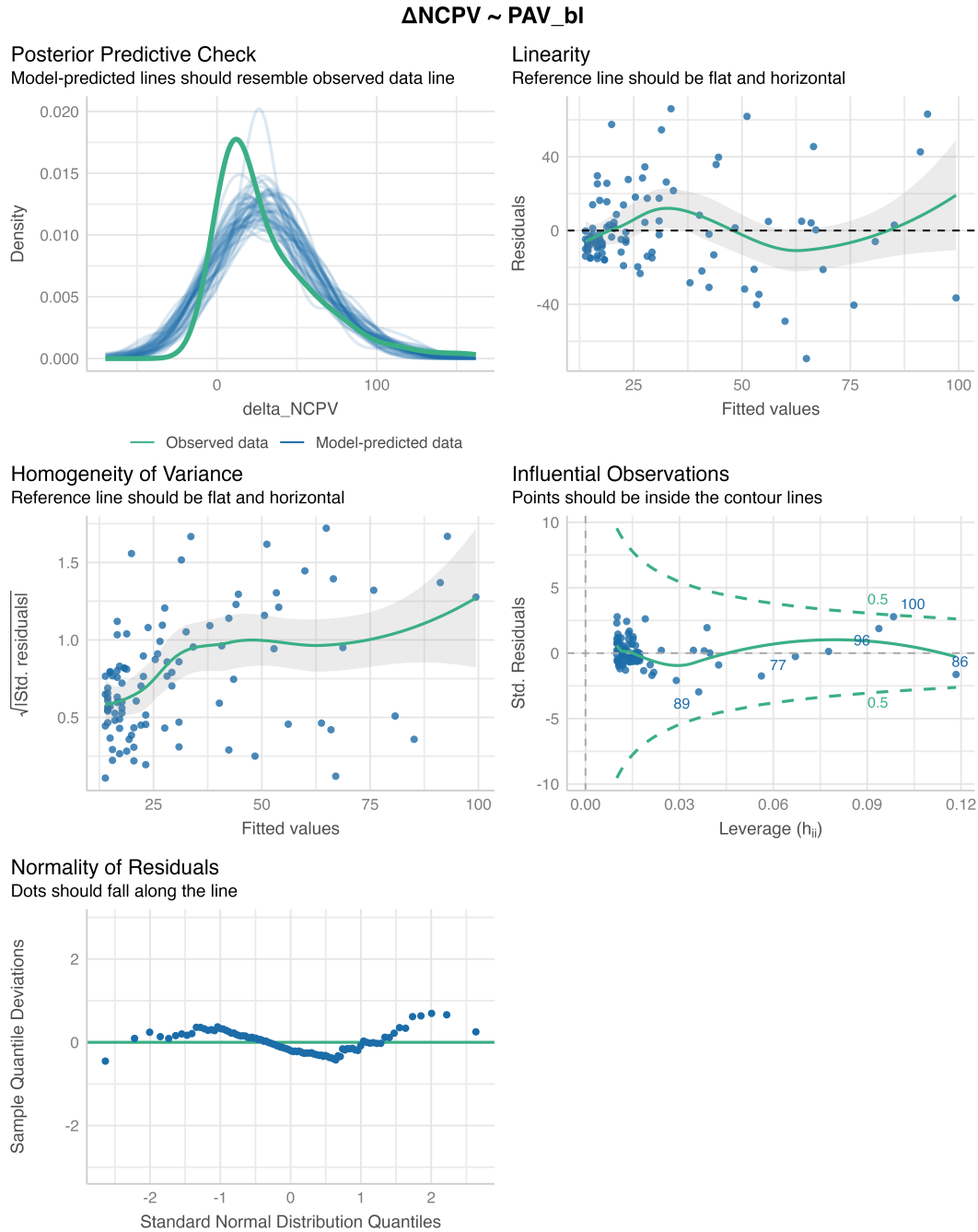
Figure 2: performance::check_model(lm( \Delta\text{NCPV} \sim \text{PAV}_{bl} )) output for the reported change-score model
