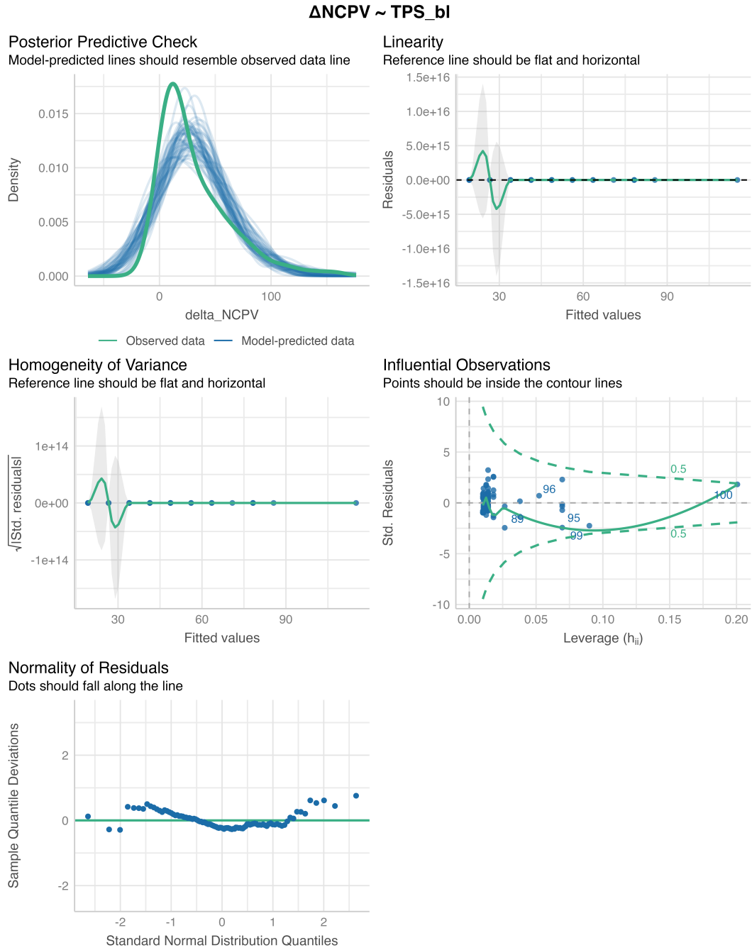
Figure 3: performance::check_model(lm( \Delta\text{NCPV} \sim \text{TPS}_{bl} )) output for the reported change-score model
