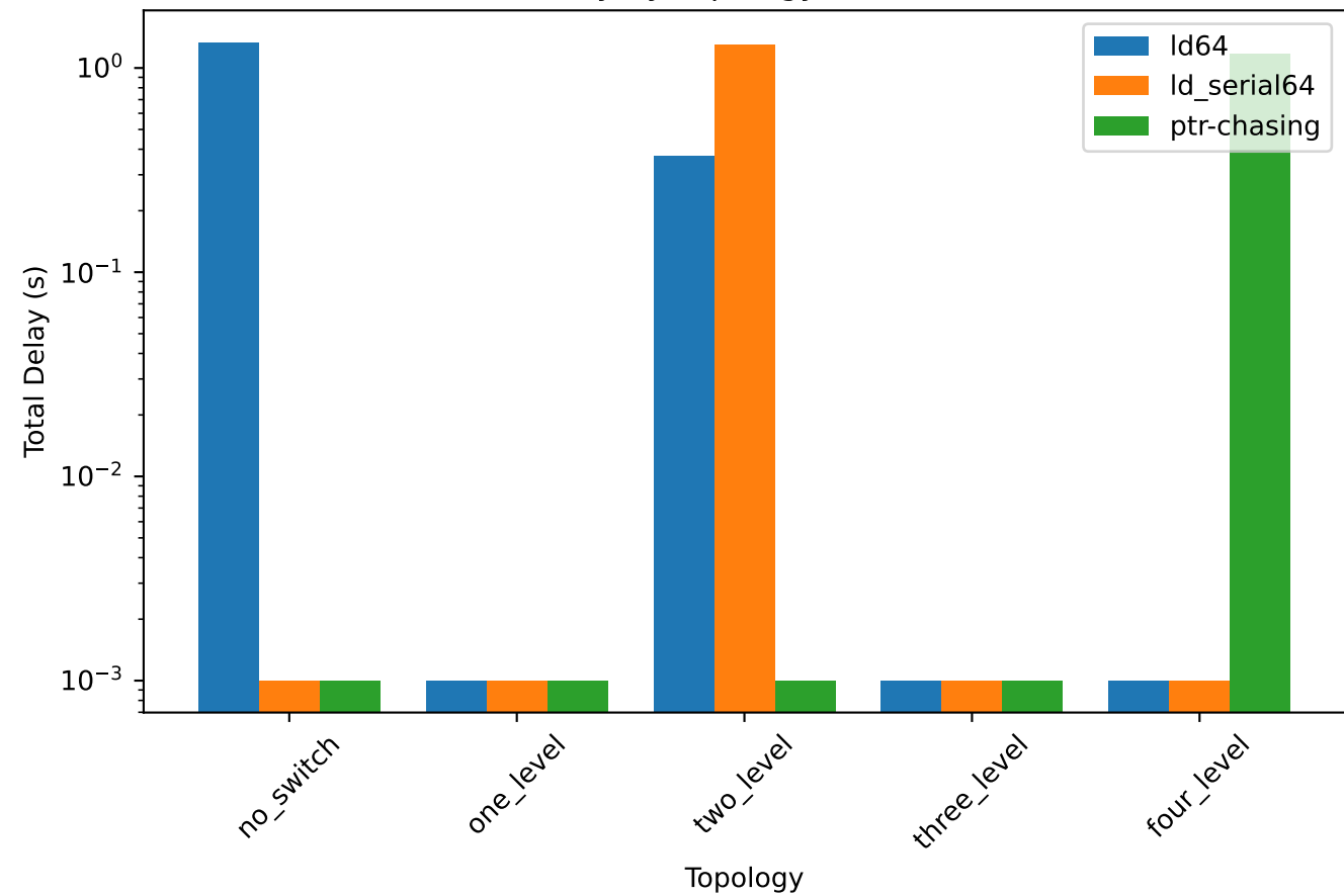
Total Delay by Topology and Workload
