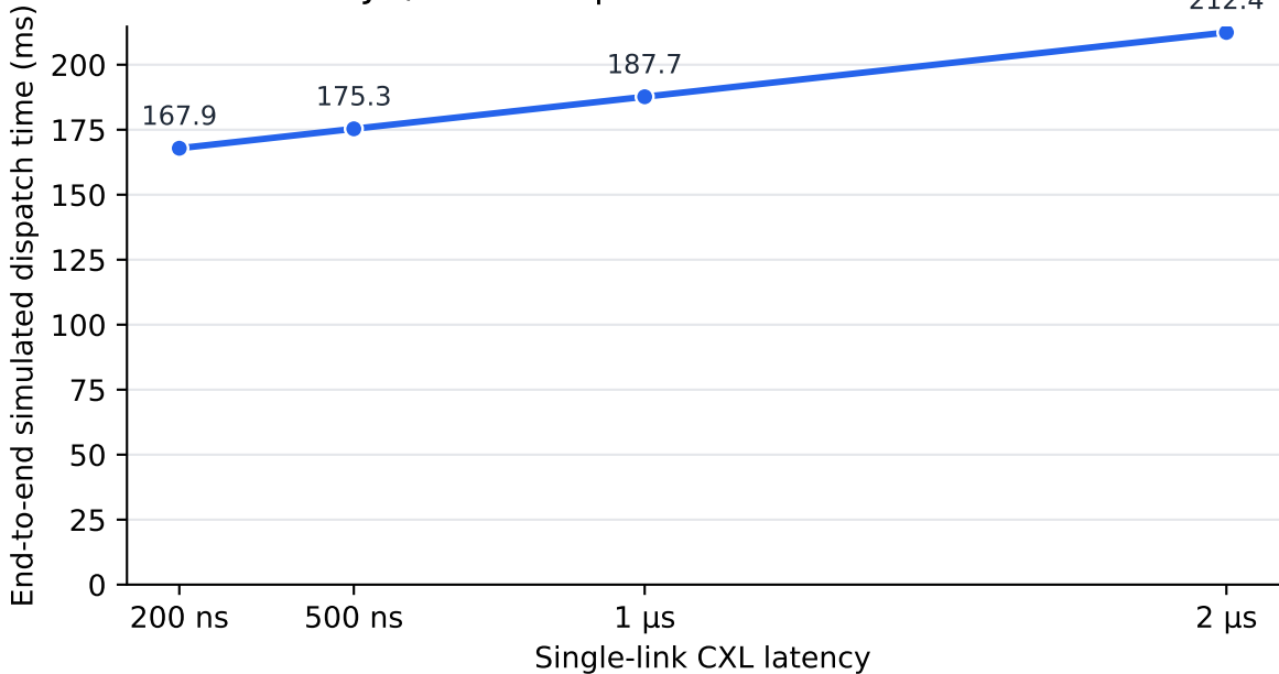
CIRA JIT/Vortex dispatch over a modeled CXL link
