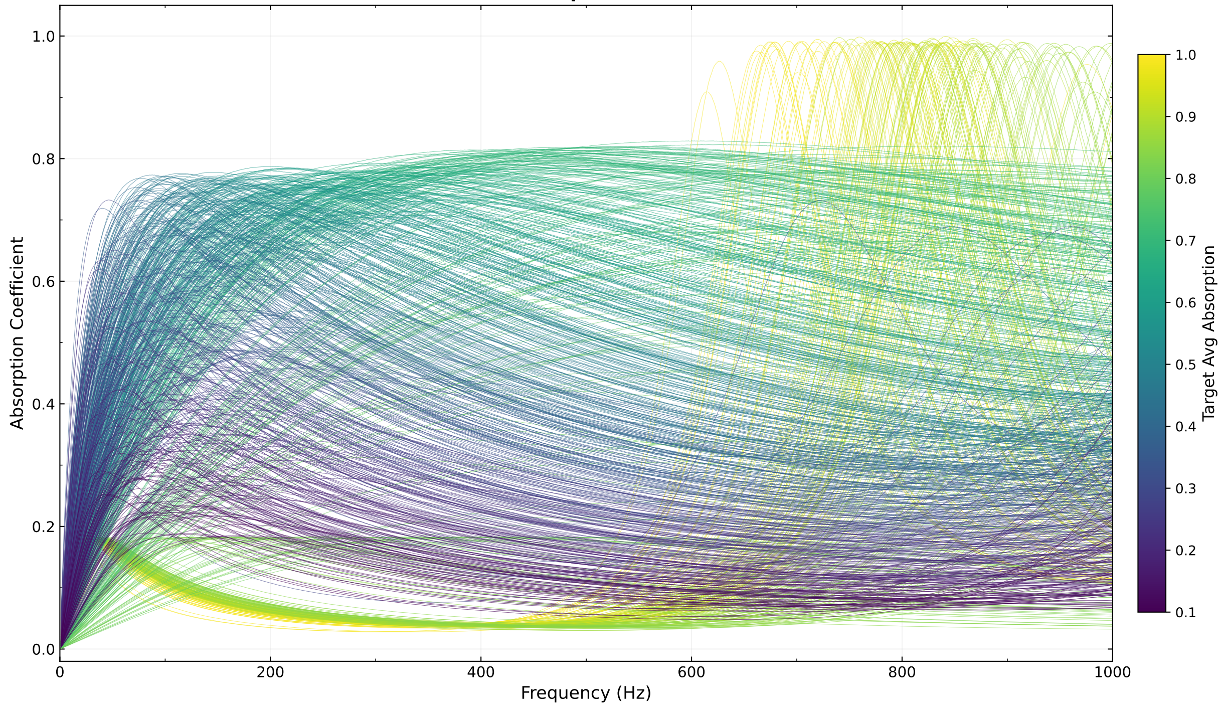
Design-Space Sweep: 901 Targets (0.1 → 1.0) Best-of-20 — Full Absorption Curves via GPU TMM
