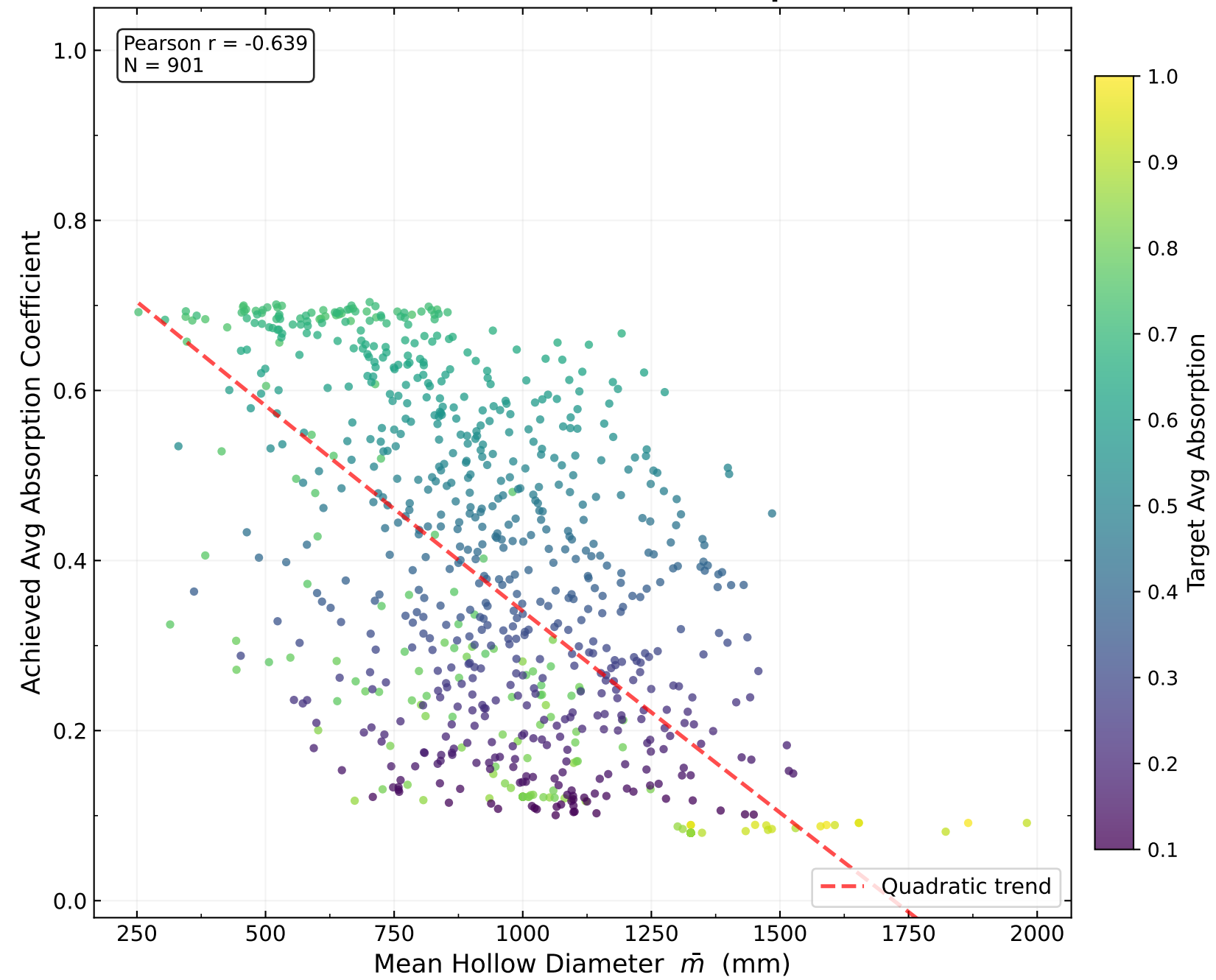
(b) Hollow Diameter vs Absorption
