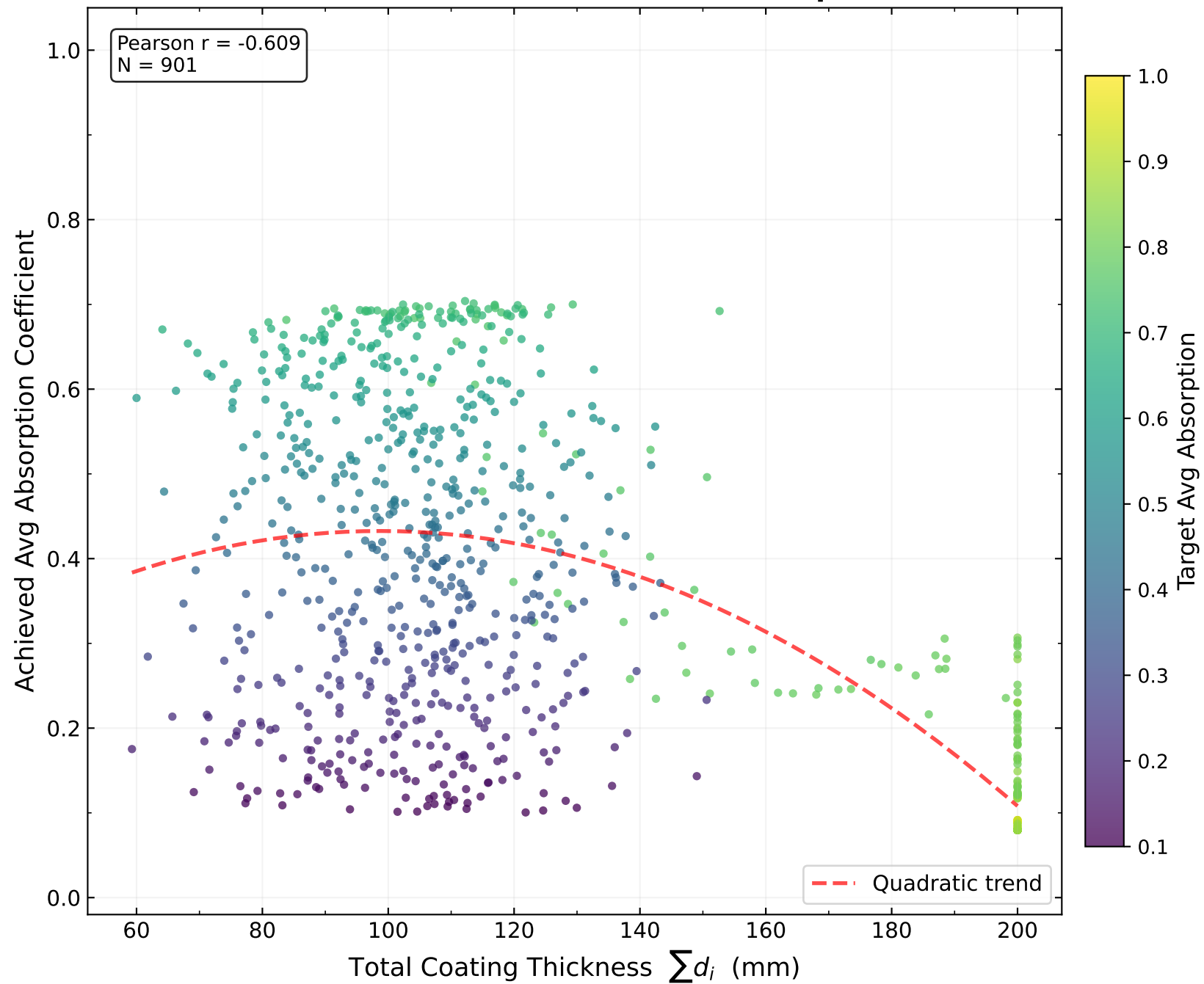
(a) Pareto Front: Thickness vs Absorption
