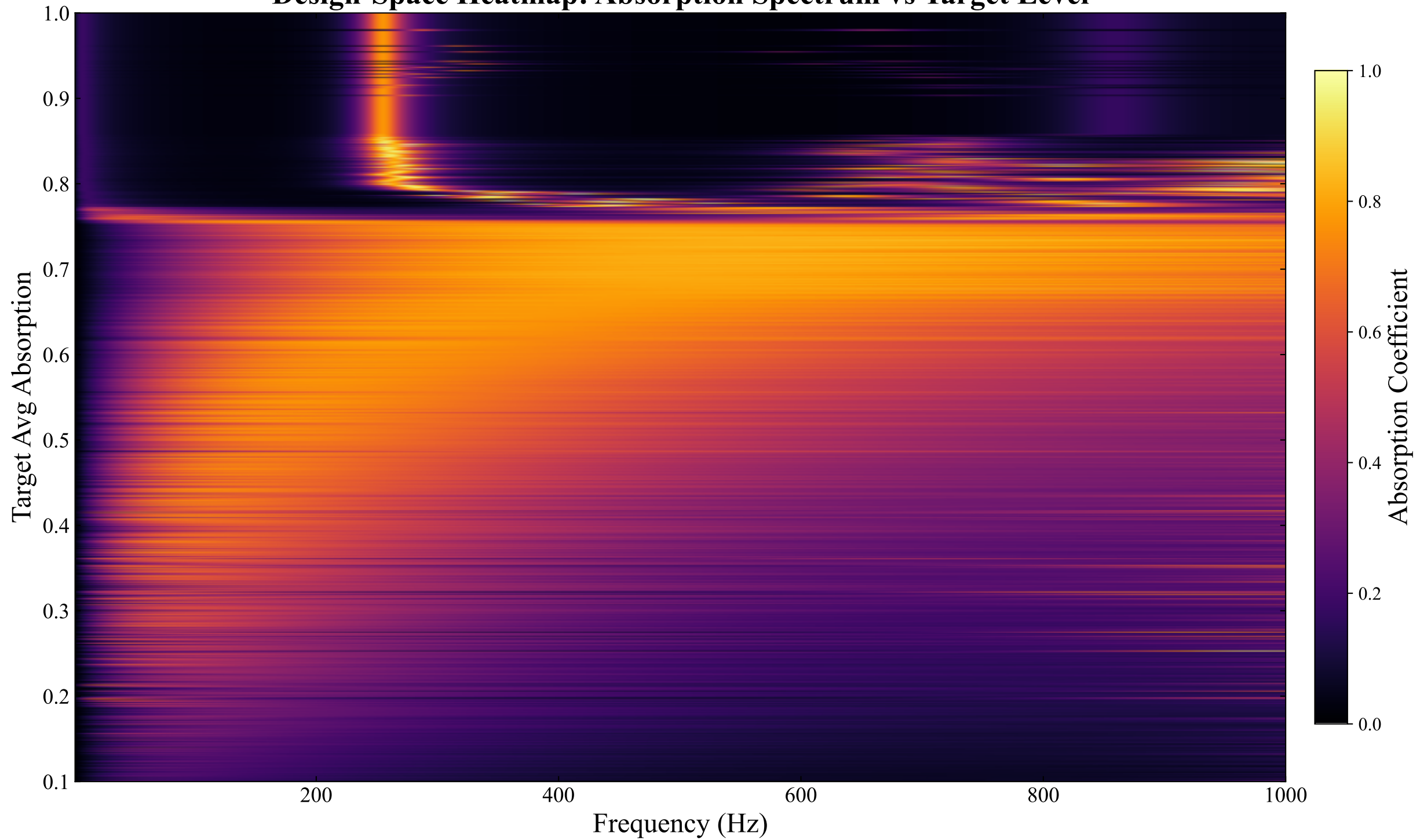
Design-Space Heatmap: Absorption Spectrum vs Target Level
