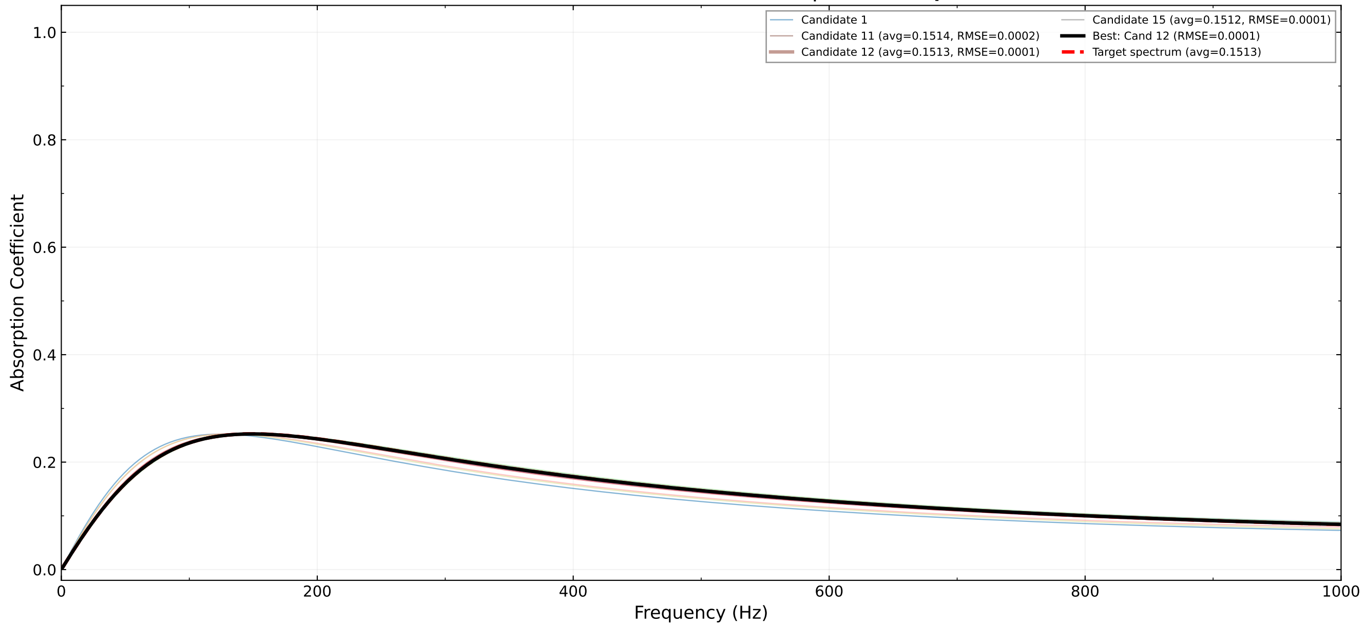
Best Test Sample (idx=48329) — All 20 Candidates Full 1-1000 Hz via Theoretical Model TMM | cINN Full-Spectrum
