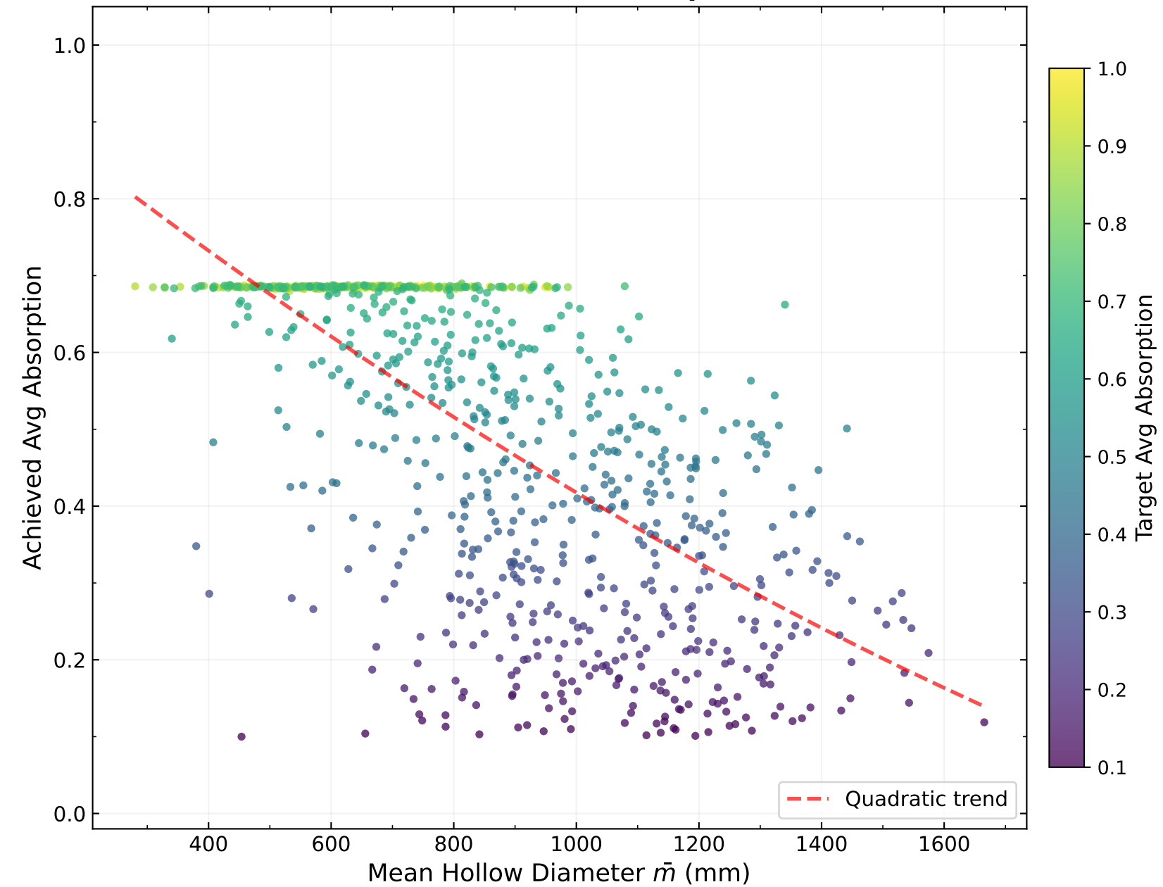
(b) Hollow Diameter vs Absorption (cINN)
