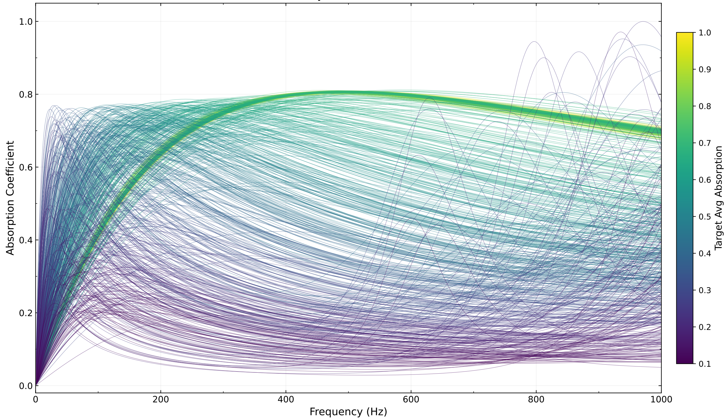
Design-Space Sweep: 901 Targets (0.1 → 1.0) Best-of-20 — Full Absorption Curves via GPU TMM (cINN)
