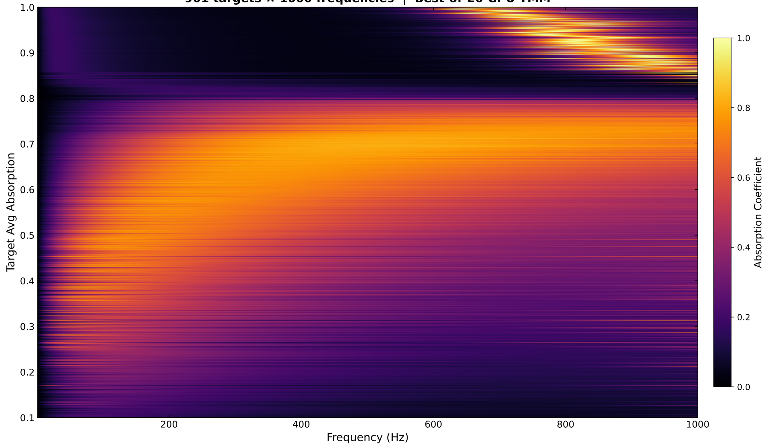
Design-Space Heatmap: Absorption Spectrum vs Target Level 901 targets × 1000 frequencies | Best-of-20 GPU TMM
