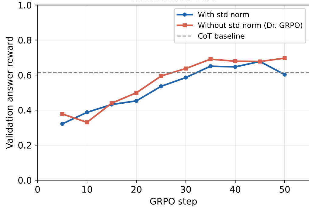
Validation Reward
