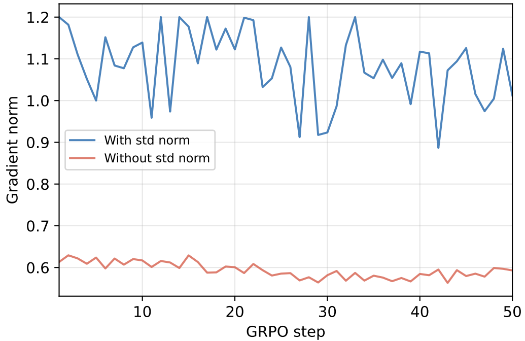
Gradient Norm Stability
