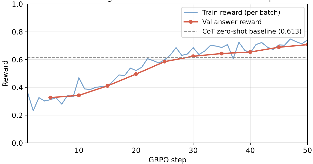
GRPO Training - Validation Answer Reward over 50 Steps
