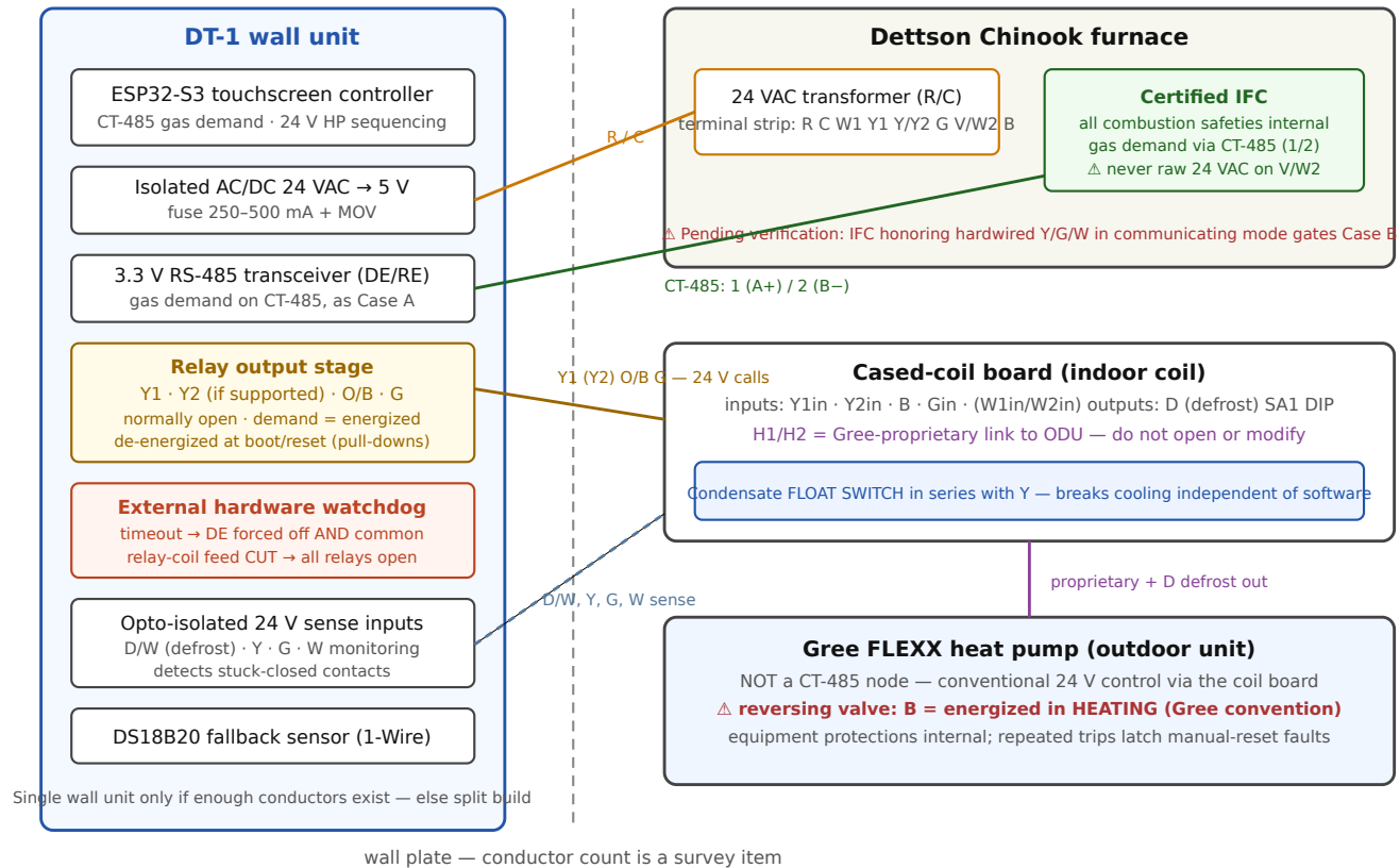
Case B — hybrid installation, block diagram
