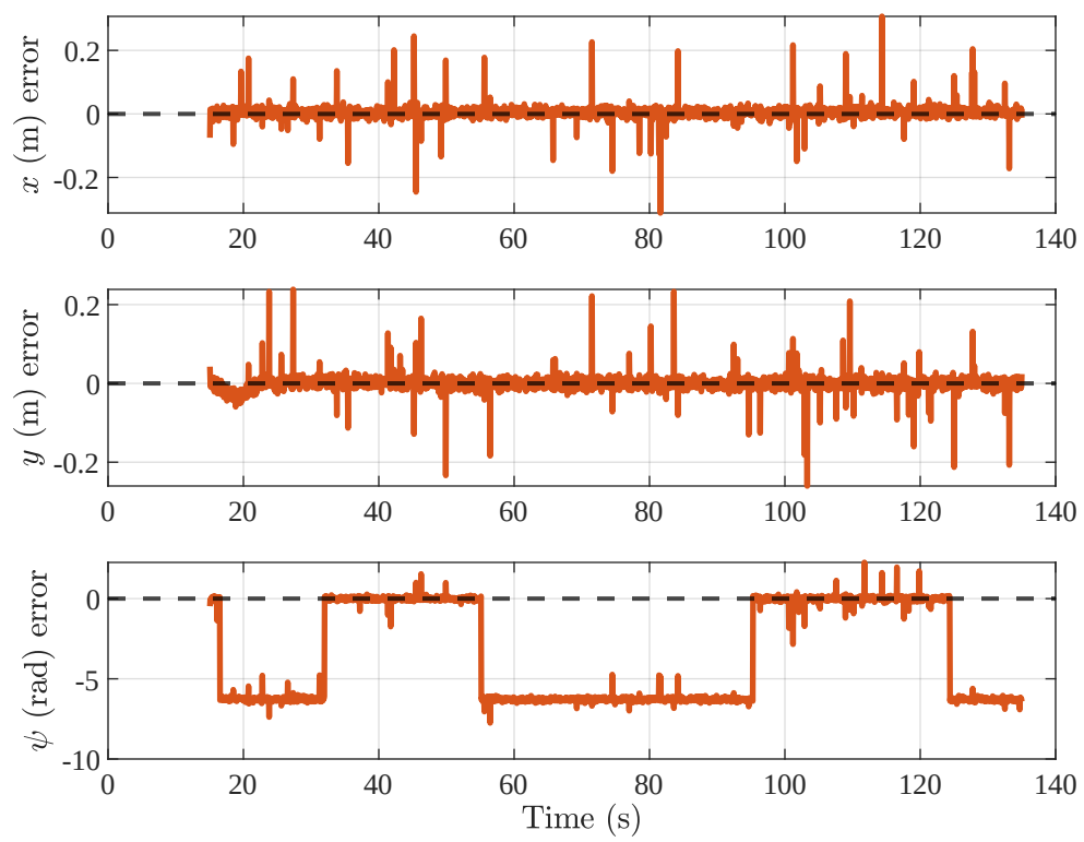
Inertial Measurement Error
