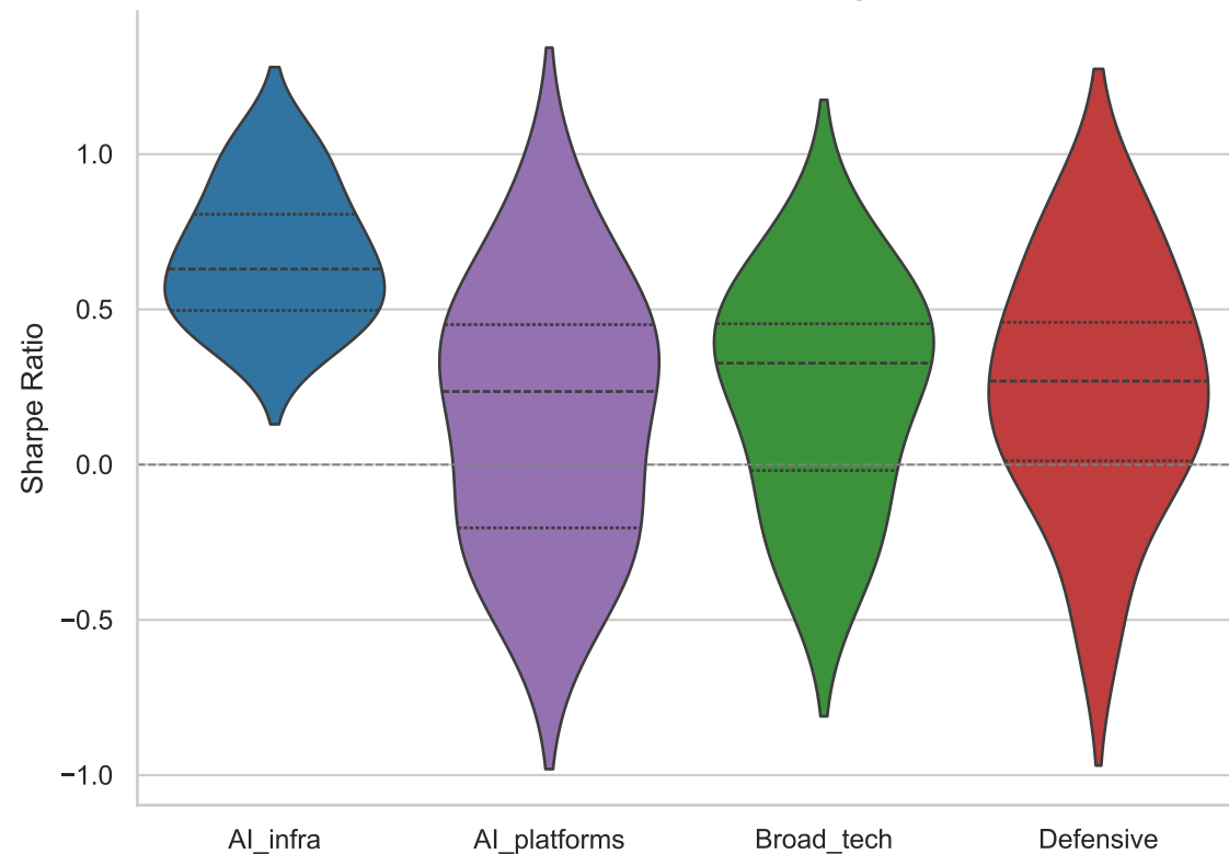
Violin plot - Sharpe Ratio per grupa
