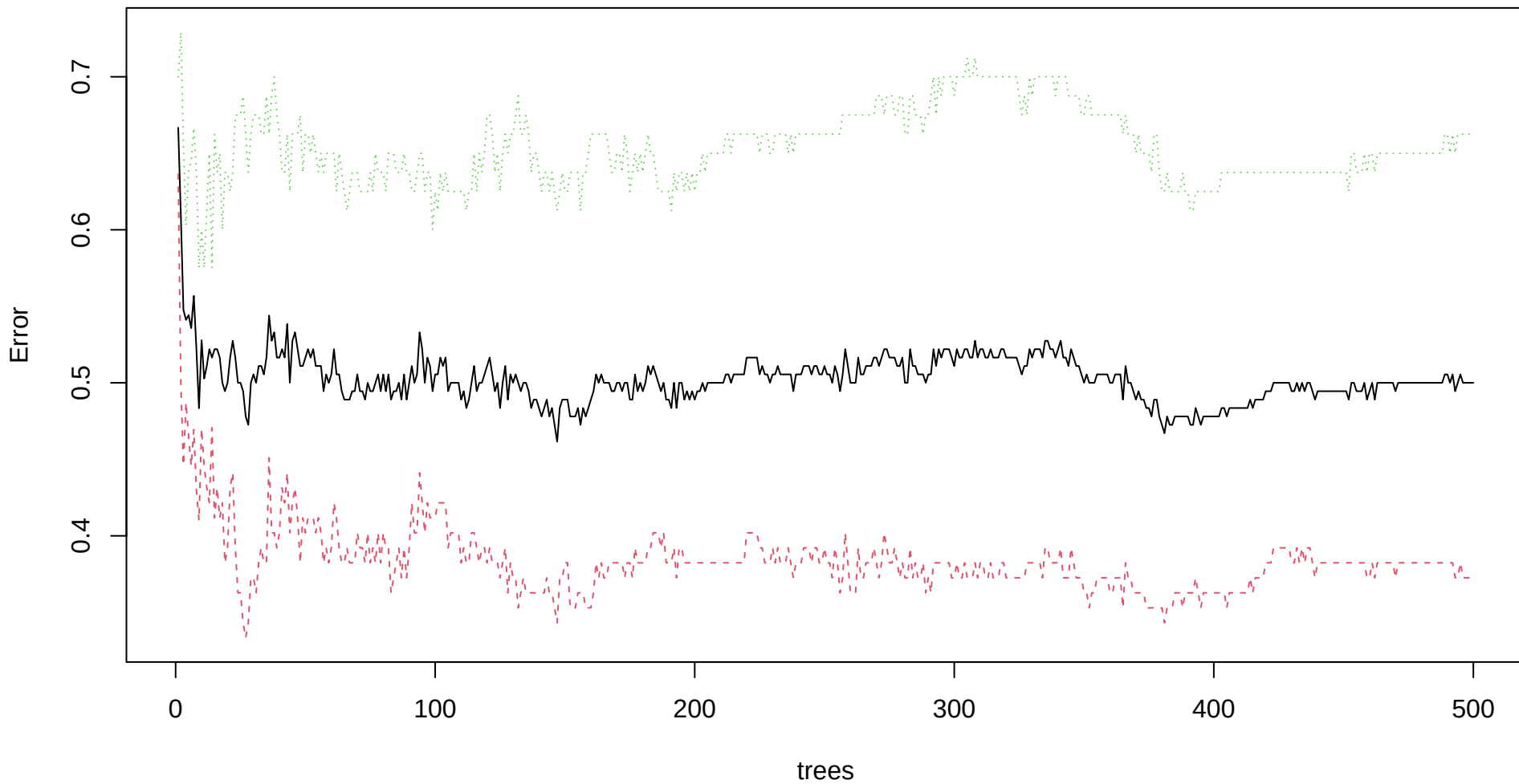
model_treatment
