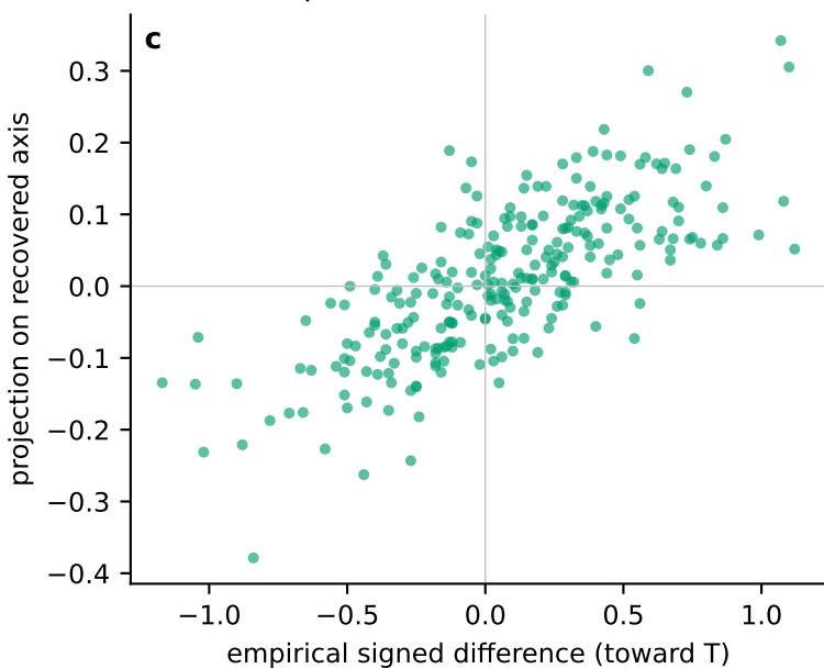
Feeling-Thinking \rho = 0.75 [0.69, 0.80]
