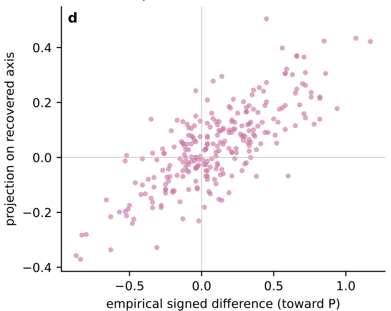
Judging-Perceiving \rho = 0.73 [0.65, 0.78]
