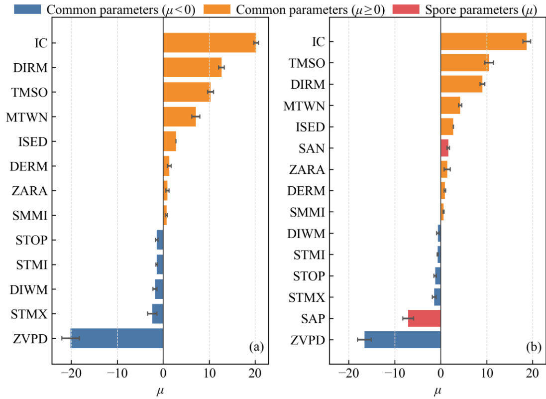
Figure 10. Signed mean effects ( \mu ) from the Morris global sensitivity analysis for the baseline FSIM model (a) and the extended FSIM-S model (b). Positive and negative values indicate the direction of parameter influence on model output, while bar length reflects effect magnitude. Results are aggregated across multiple random seeds, with error bars representing variability among runs.
