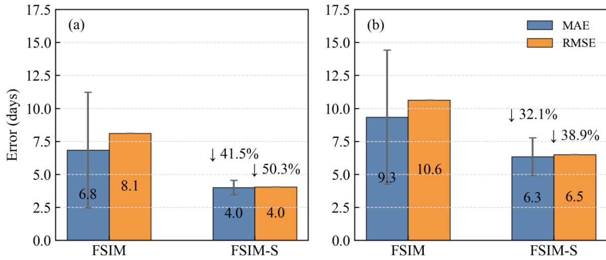
Figure 11. Model performance comparison based on mean absolute error (MAE) and root mean square error (RMSE): (a) training set and (b) test set. Bars show mean errors (days) \pm standard deviations across folds. The percentages denote relative error reductions compared with the baseline FSIM model.
