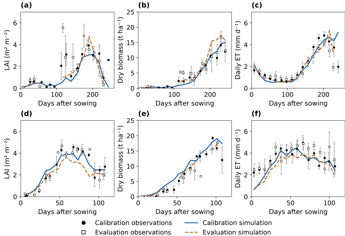
405 Figure 4. Multisite seasonal crop comparisons. Wheat and maize occupy the top and bottom rows; columns show LAI, aboveground 406 dry biomass and daily actual ET. Filled and open observations distinguish the original calibration and retrospective-evaluation 407 partitions; solid blue and dashed orange lines show the corresponding simulations. Error bars describe standard errors among site- 408 year means. Balanced means use 15-day wheat and seven-day maize bins, and unobserved bins remain gaps. Accuracy scores use 409 unbinned records. Complete station irrigation management remains unconfirmed.
