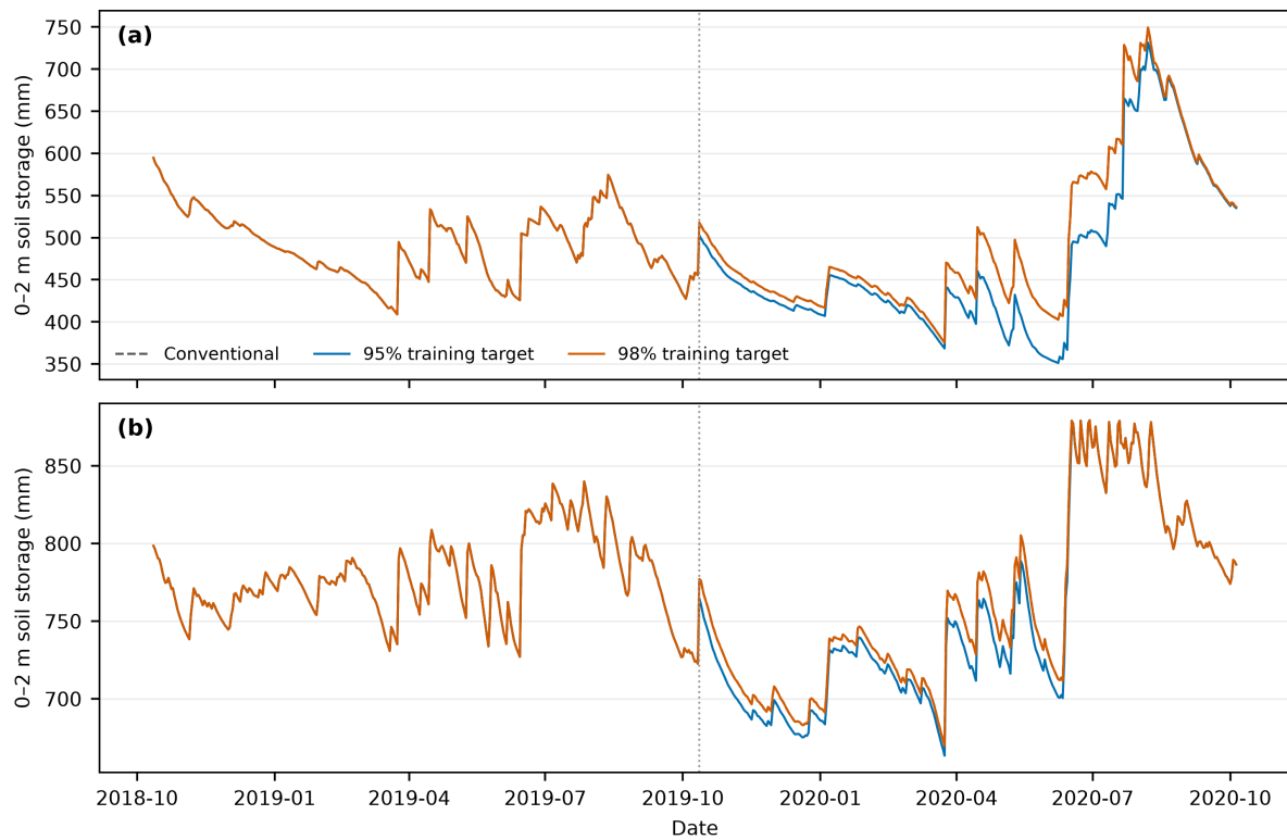
233 Figure S3. Simulated 0–2 m soil-water storage in representative units (a) 0 and (b) 31. State carries continuously through wheat, 234 maize, fallows and annual irrigation choices. Displayed histories compare conventional irrigation with selected current strategies; 235 they are model states rather than observed groundwater levels.
