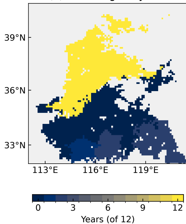
(e) Positive grain years
