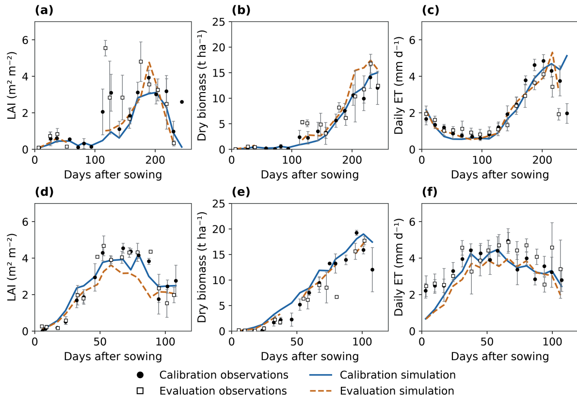
418 Figure 5. Multisite seasonal crop comparisons. Wheat and maize occupy the top and bottom rows; columns show LAI, aboveground 419 dry biomass and daily actual ET. Filled and open observations distinguish the original calibration and retrospective-evaluation 420 partitions; solid blue and dashed orange lines show the corresponding simulations. Error bars describe standard errors among site- 421 year means. Balanced means use 15-day wheat and seven-day maize bins, and unobserved bins remain gaps. Accuracy scores use 422 unbinned records. Complete station irrigation management remains unconfirmed.
