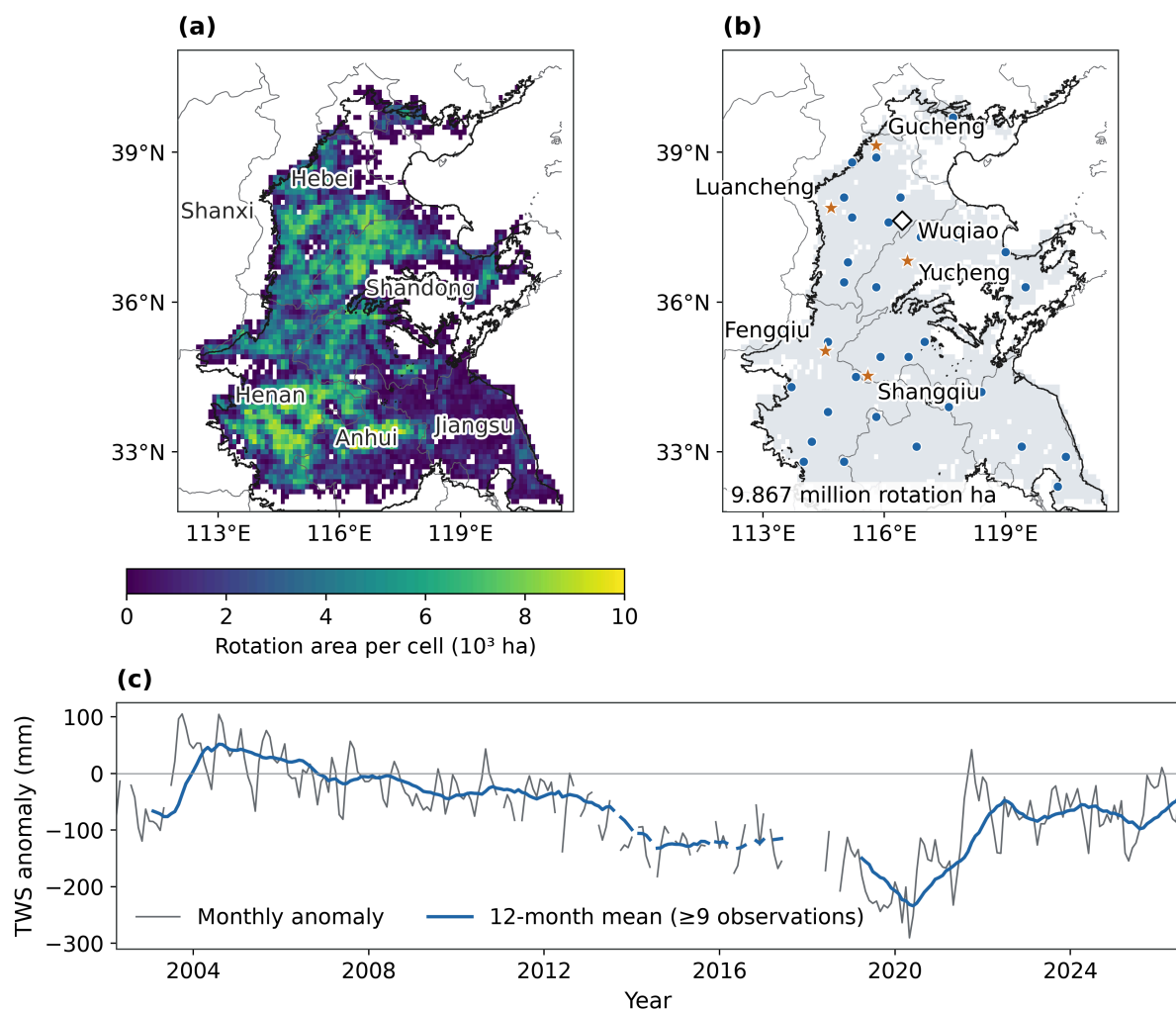
136 Figure 2. Study domain, rotation area, observation sites and regional water storage. (a) Mapped 2020 wheat–maize rotation area. (b) 137 Five crop-observation sites, the Wuqiao irrigation experiment and 32 regional simulation units. (c) Observed CSR monthly 138 terrestrial-water-storage anomalies and a 12-calendar-month mean requiring at least nine observations. Missing months remain 139 gaps. Thin grey lines show provincial boundaries; black outlines delimit the operational physiographic study domain. Maps use an 140 equiarectangular projection (36°N, 117°E). Provincial boundaries: Natural Earth Admin 1 v5.1.1 (Natural Earth, n.d.).
