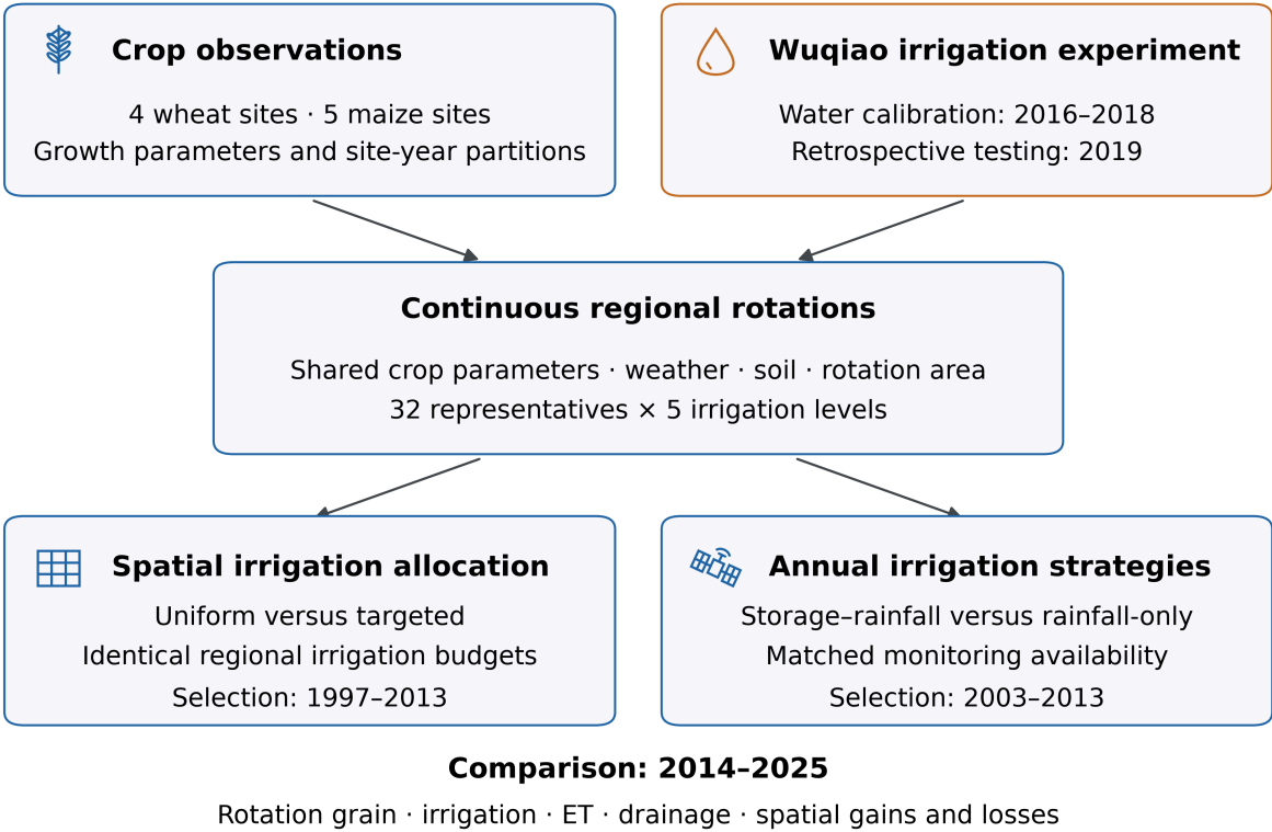
118 Figure 1. Study workflow. Multisite observations support growth parameters, while documented Wuqiao treatments calibrate water- 119 use parameters and provide retrospective testing. Shared parameters drive continuous regional rotations. Spatial allocation 120 compares uniform and targeted irrigation under identical budgets; annual strategies compare storage–rainfall and rainfall-only 121 selection under matched monitoring availability. Outcomes cover 2014–2025.
