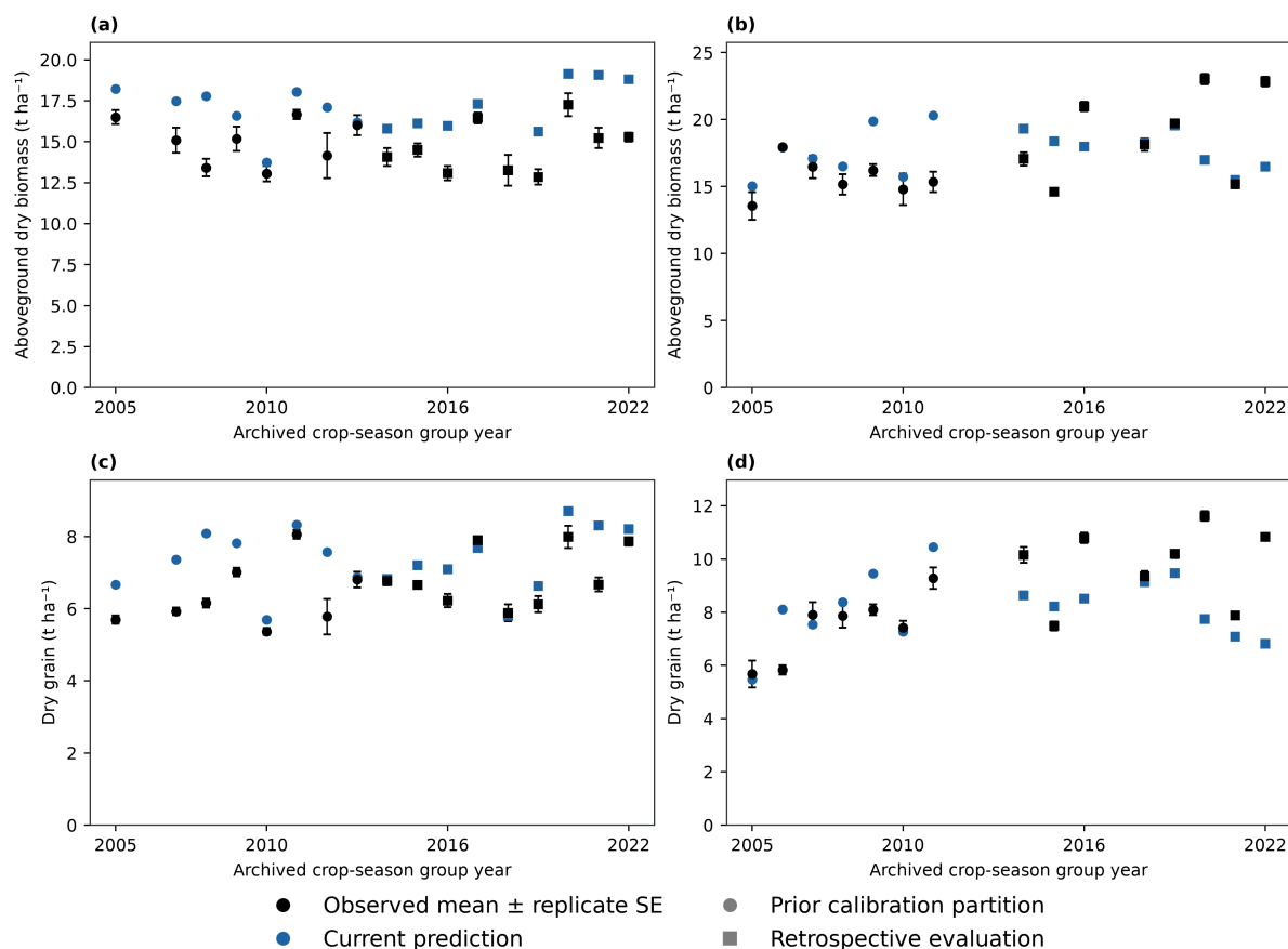
965 Figure S5. Conditional Yucheng harvest comparisons. Wheat occupies the left column and maize the right; the top row shows 966 aboveground biomass and the bottom row grain. Black points show observed means \pm standard errors among six quadrat samples 967 per crop-year; blue points show current coupled-model predictions at the same sampling windows. Circles and squares distinguish 968 the original calibration and retrospective-evaluation partitions. Grain and total aboveground biomass are dry matter. The duplicated 969 maize 2012 and 2017 source vectors remain excluded. Within-year replicates describe spatial sampling variation and are not 970 independent crop seasons. Management completeness remains unconfirmed and current water coefficients use Wuqiao fitting targets, 971 while growth coefficients retain their earlier multisite fitting history.
