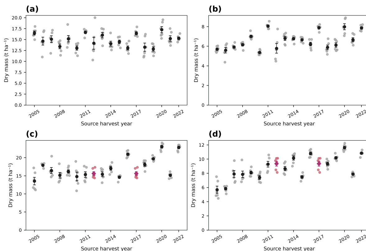
939 Figure S4. Original Yucheng harvest observations at YCAZH01ABC_01. Panels (a, b) show wheat aboveground biomass and grain; 940 panels (c, d) show maize aboveground biomass and grain. Faint points are six quadrat observations; dark markers and error bars 941 are means \pm replicate standard error. Magenta diamonds identify the identical full maize source vectors in 2012 and 2017. Raw 942 values remain displayed for source inspection; both groups are excluded from comparisons with quality-controlled observations. 943 Error bars describe sampling variation, rather than model or policy uncertainty.
