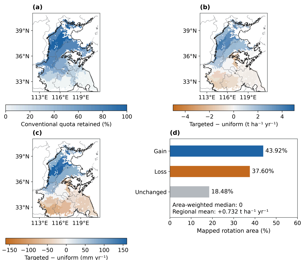
504 Figure 8. Spatial redistribution at a common 50% regional irrigation reduction, 2014–2025. (a) Targeted fraction of the conventional 505 quota; uniform allocation retains 50% everywhere. (b,c) Targeted-minus-uniform combined rotation dry grain and crop-plus-fallow 506 ET. (d) Mapped rotation-area shares with positive, negative or unchanged mean grain contrasts. The 3,641 cells inherit 32 507 representative responses. Thin grey provincial lines and black study-domain outlines follow Figure 2; unmapped areas remain blank.
