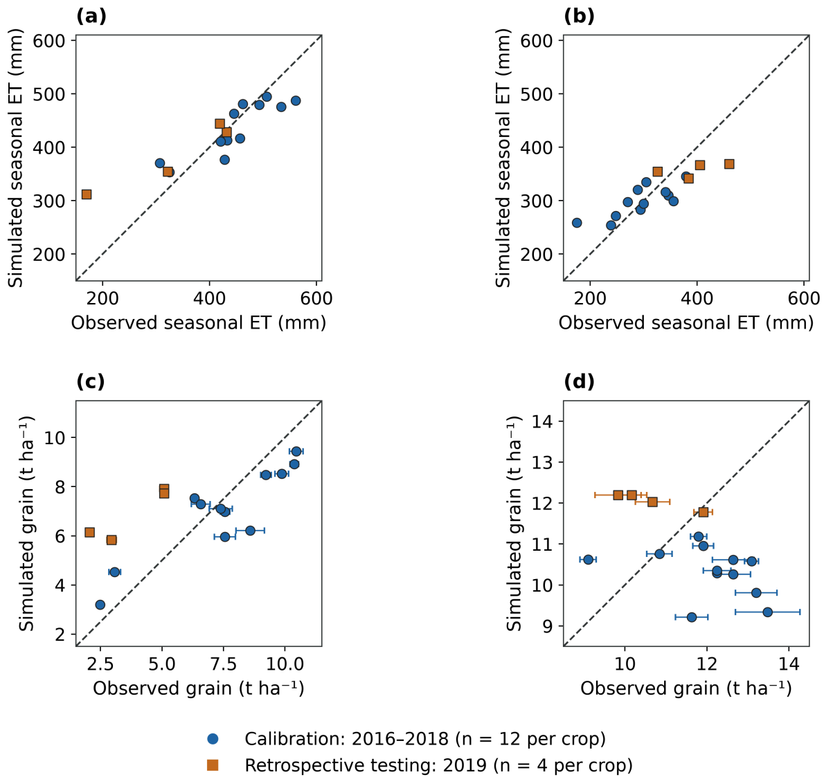
448 Figure 6. Wuqiao calibration and retrospective testing. (a,b) Seasonal ET; (c,d) annual treatment-mean grain at 13% moisture. 449 Wheat occupies the left column and maize the right. Circles show 2016–2018 treatments used to fit water-use parameters; squares 450 show 2019, withheld from the fit and selection. Dashed lines denote 1:1 agreement. Crop-specific grain axes focus on their observed 451 ranges. Horizontal grain error bars are the published SE from three field replicates. Observed ET follows the published 0–2 m water 452 balance; simulated dry grain is converted once by division by 0.87. Maize labels retain preceding wheat management with identical 453 maize irrigation within each year.
