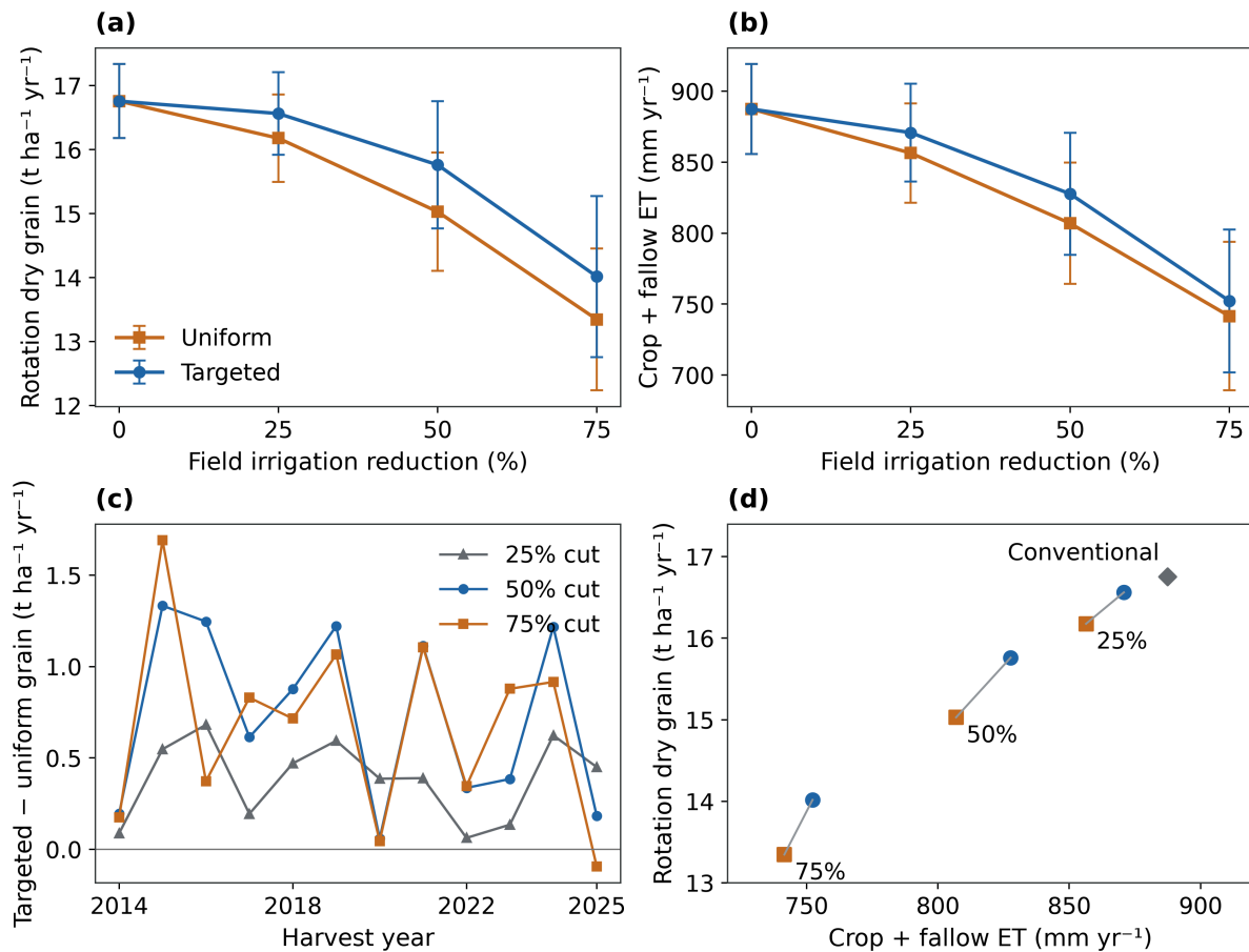
Figure 6. Irrigation allocation and grain–water trade-offs during 2014–2025. (a,b) Rotation-area-weighted annual combined wheat–maize dry grain and crop-plus-fallow ET; error bars are between-year SD. (c) Annual targeted-minus-uniform grain at identical irrigation budgets. (d) Period means; connectors join policies with the same budget. Values per hectare use the same 9.867 million mapped rotation hectares, rather than separate crop areas. Targeting retains more grain than uniform cuts while remaining below conventional production.
