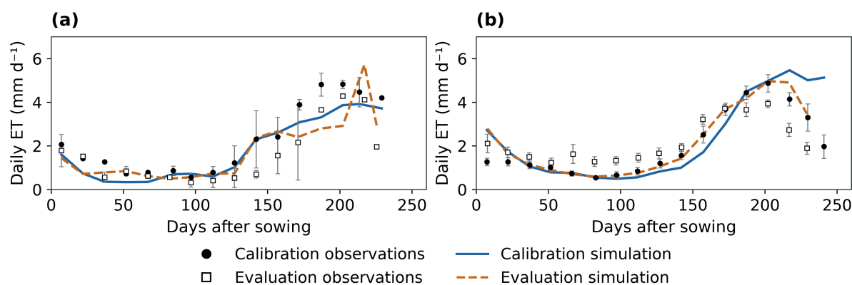
938 Figure S8. Site-specific wheat ET comparisons: (a) Fengqiu; (b) Yucheng. Calibration and retrospective-evaluation observations and 939 simulations share the same axes within each site. Error bars describe site-year standard errors; gaps are retained. The observations, 940 weighting and conditional management interpretation follow Figure 4.
