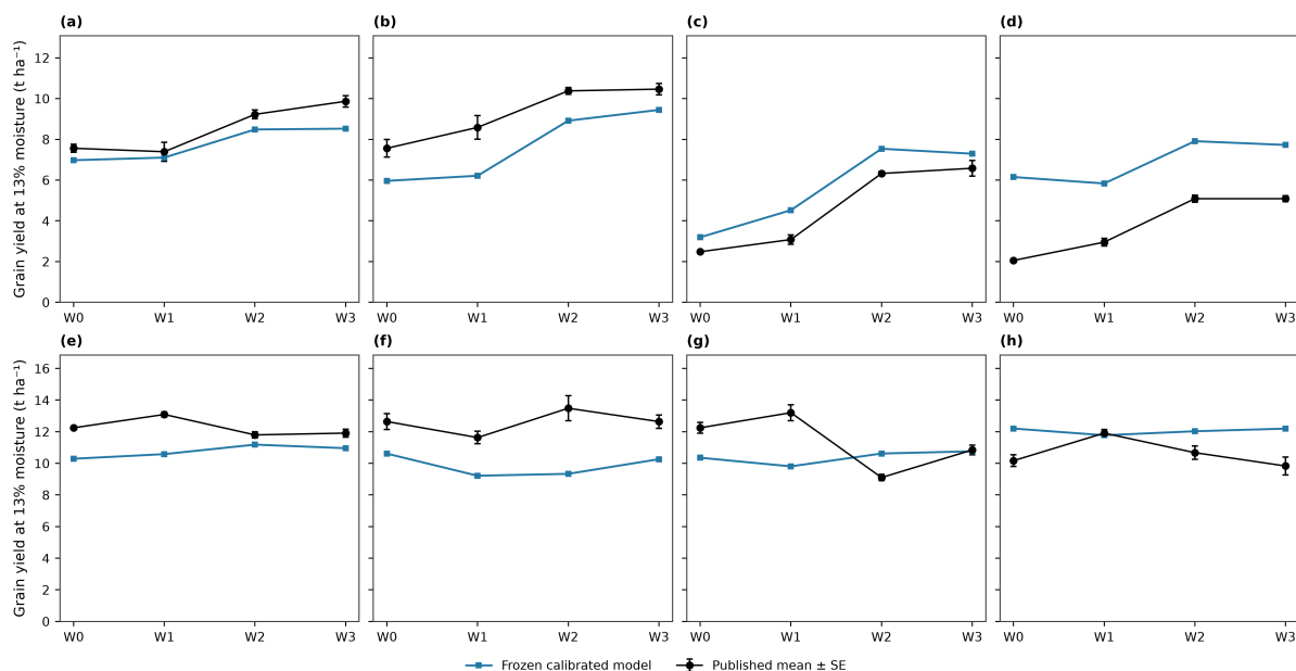
868 Figure S2. Annual Wuqiao grain at 13% moisture under the selected current parameters. Panels (a–d) show wheat and (e–h) maize; 869 columns from left to right show 2016, 2017, 2018 and 2019. Black points and error bars are published means \pm standard error of 870 three replicates; blue squares show current predictions. The 2016–2018 treatment means contribute to water calibration after 871 conversion to dry grain; 2019 is retrospective testing, excluded from fitting and selection. Maize irrigation is identical within each 872 year and labels retain preceding wheat management. Source means and SE are digitized from Supplementary Figure S2 of the 873 primary experiment.
