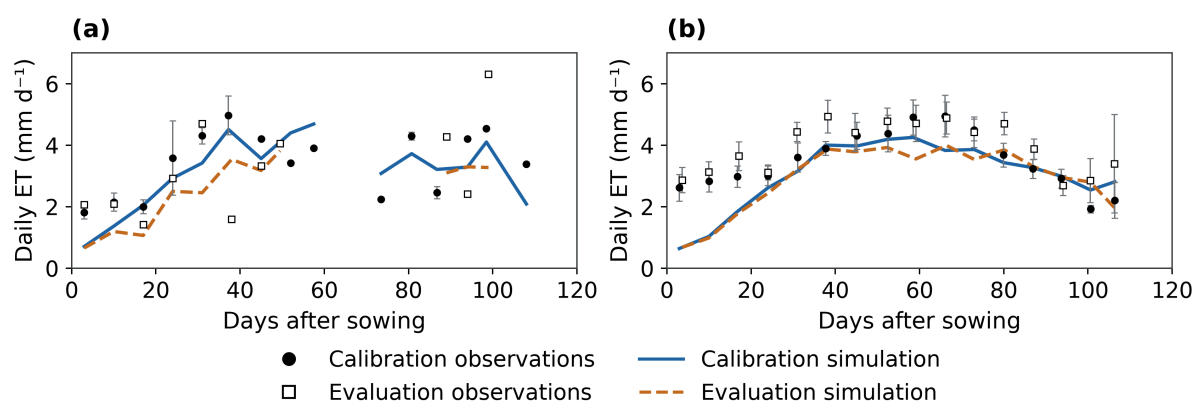
947 Figure S11. Site-specific maize ET comparisons: (a) Fengqiu; (b) Yucheng. Calibration and retrospective-evaluation observations and 948 simulations share the same axes within each site. Error bars describe site-year standard errors; gaps are retained. The observations, 949 weighting and conditional management interpretation follow Figure 4.
