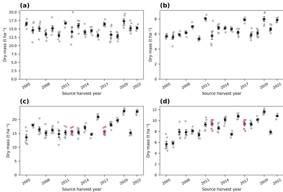
899 Figure S4. Original Yucheng harvest observations at YCAZH01ABC_01. Panels (a, b) show wheat aboveground biomass and grain; panels (c, d) show maize aboveground biomass and grain. Faint points are six quadrat observations; dark markers and error bars are means \pm replicate standard error. Magenta diamonds identify the identical full maize source vectors in 2012 and 2017. Raw values remain displayed for source inspection; both groups are excluded from comparisons with quality-controlled observations. Error bars describe sampling variation, rather than model or policy uncertainty.
