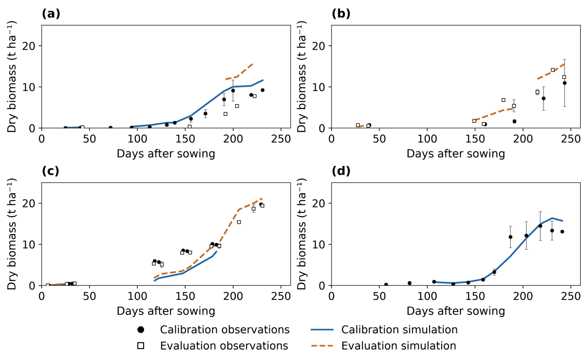
935 Figure S7. Site-specific wheat aboveground biomass comparisons: (a) Fengqiu; (b) Luancheng; (c) Shangqiu; (d) Yucheng. 936 Calibration and retrospective-evaluation observations and simulations share the same axes within each site. Error bars describe site- 937 year standard errors; gaps are retained. The observations, weighting and conditional management interpretation follow Figure 4.
