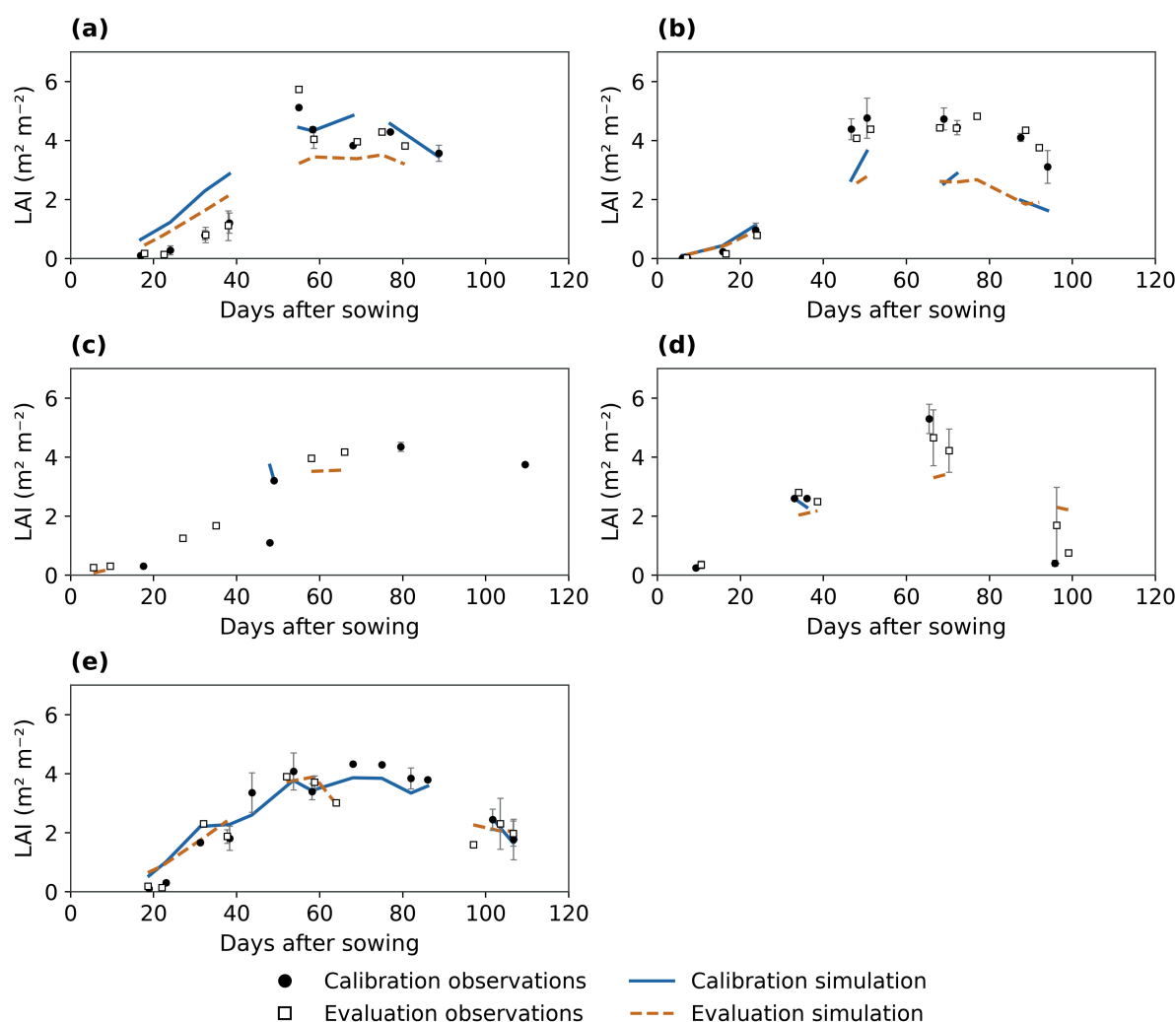
941 Figure S9. Site-specific maize LAI comparisons: (a) Fengqiu; (b) Gucheng; (c) Luancheng; (d) Shangqiu; (e) Yucheng. Calibration 942 and retrospective-evaluation observations and simulations share the same axes within each site. Error bars describe site-year 943 standard errors; gaps are retained. The observations, weighting and conditional management interpretation follow Figure 4.
