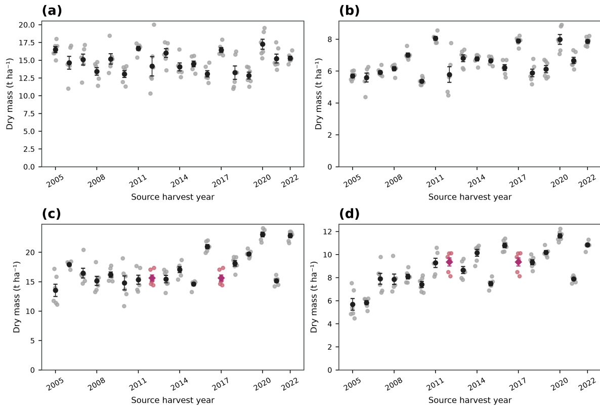
274 Figure S4. Original Yucheng harvest observations at YCAZH01ABC_01. Panels (a, b) show wheat aboveground biomass and grain; 275 panels (c, d) show maize aboveground biomass and grain. Faint points are six quadrat observations; dark markers and error bars 276 are means \pm replicate standard error. Magenta diamonds identify the identical full maize source vectors in 2012 and 2017. Raw 277 values remain displayed for source inspection; both groups are excluded from comparisons with quality-controlled observations. 278 Error bars describe sampling variation, rather than model or policy uncertainty.
