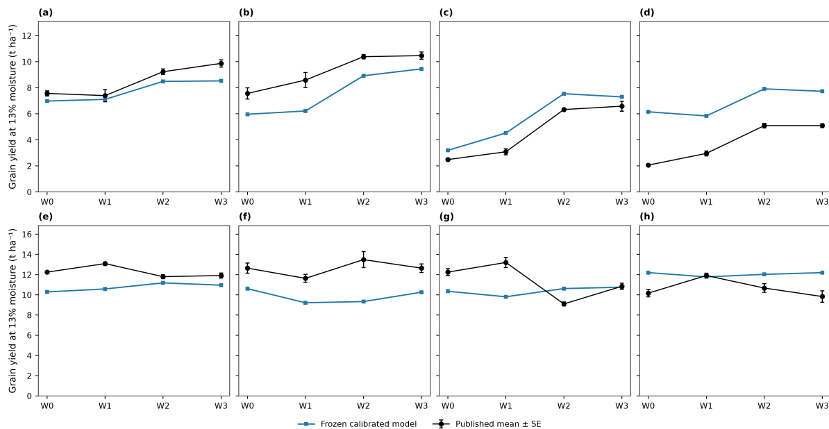
243 Figure S2. Annual Wuqiao grain at 13% moisture under the selected current parameters. Panels (a–d) show wheat and (e–h) maize; 244 columns from left to right show 2016, 2017, 2018 and 2019. Black points and error bars are published means \pm standard error of 245 three replicates; blue squares show current predictions. The 2016–2018 treatment means contribute to water calibration after 246 conversion to dry grain; 2019 is retrospective testing, excluded from fitting and selection. Maize irrigation is identical within each 247 year and labels retain preceding wheat management. Source means and SE are digitized from Supplementary Figure S2 of the 248 primary experiment.
