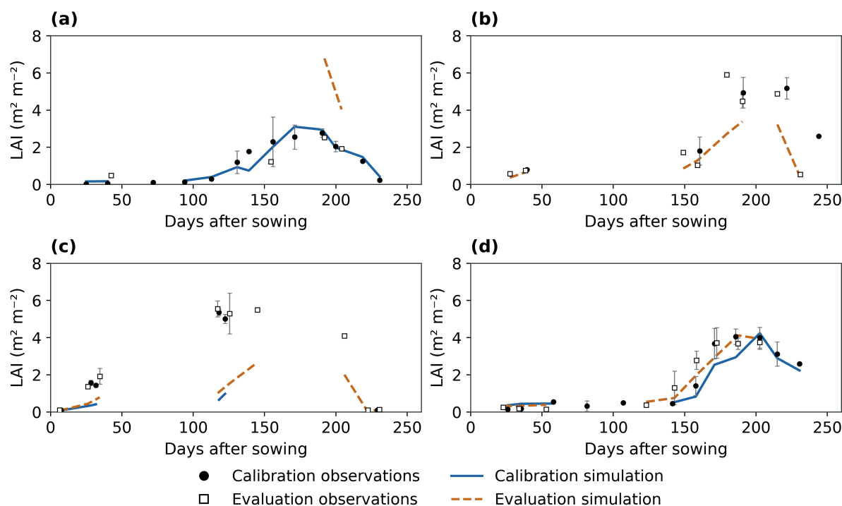
307 Figure S6. Site-specific wheat LAI comparisons: (a) Fengqiu; (b) Luancheng; (c) Shangqiu; (d) Yucheng. Calibration and 308 retrospective-evaluation observations and simulations share the same axes within each site. Error bars describe site-year 309 errors; gaps are retained. The observations, weighting and conditional management interpretation follow Figure 6.
