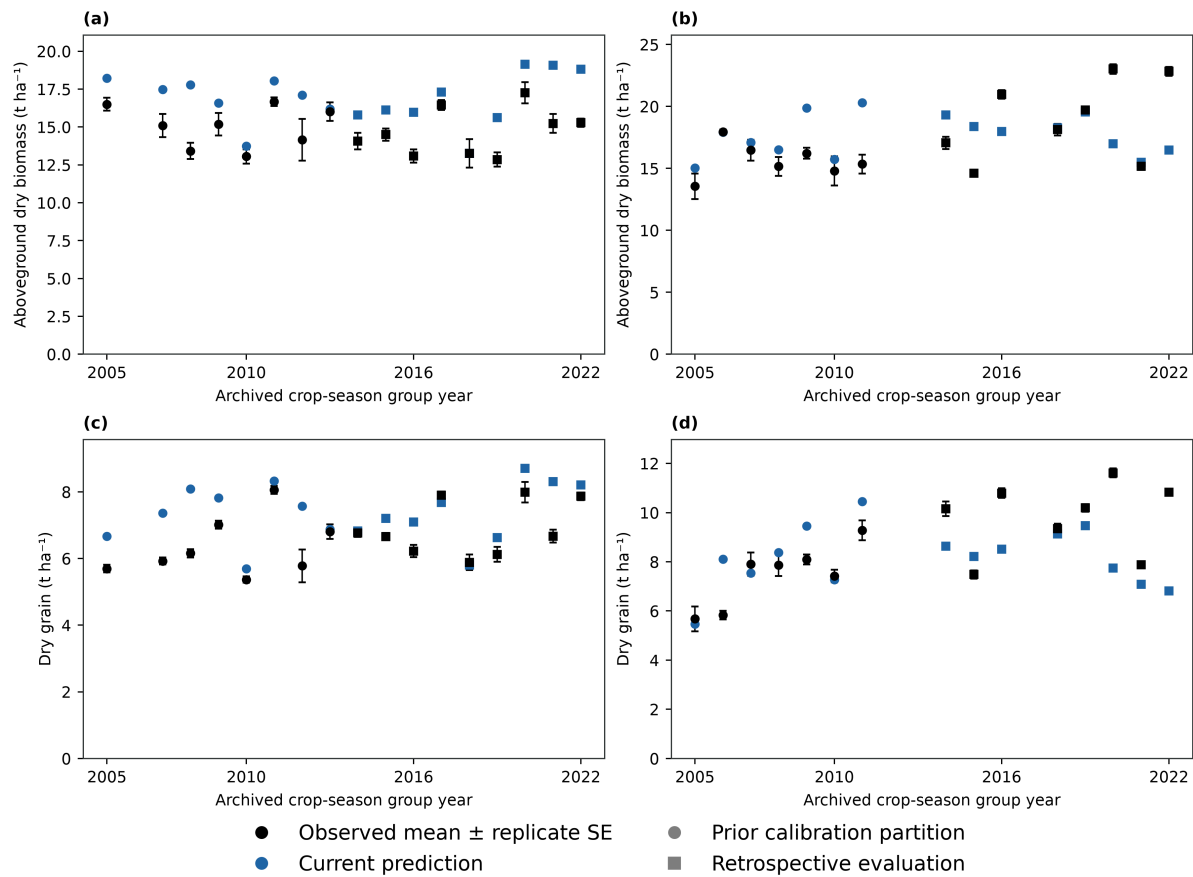
300 Figure S5. Conditional Yucheng harvest comparisons. Wheat occupies the left column and maize the right; the top row shows 301 aboveground biomass and the bottom row grain. Black points show observed means \pm standard errors among six quadrat samples 302 per crop-year; blue points show current coupled-model predictions at the same sampling windows. Circles and squares distinguish 303 the original calibration and retrospective-evaluation partitions. Grain and total aboveground biomass are dry matter. The duplicated 304 maize 2012 and 2017 source vectors remain excluded. Within-year replicates describe spatial sampling variation and are not 305 independent crop seasons. Management completeness remains unconfirmed and current water coefficients use Wuqiao fitting targets, 306 while growth coefficients retain their earlier multisite fitting history.
