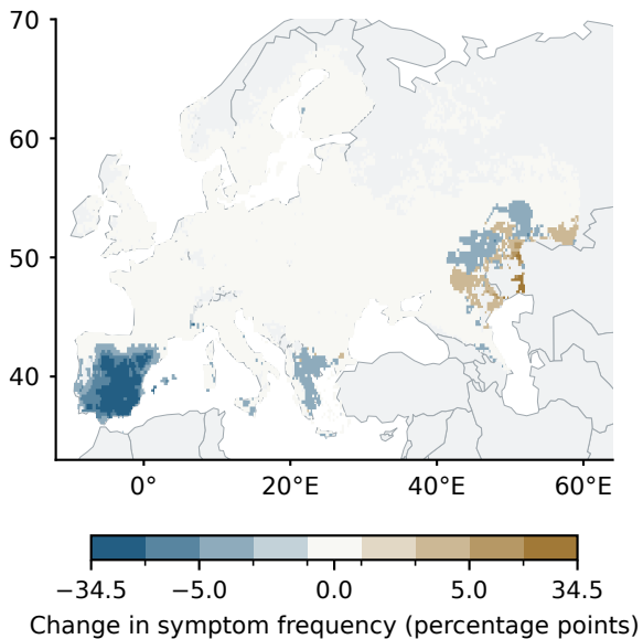
a Symptom frequency
