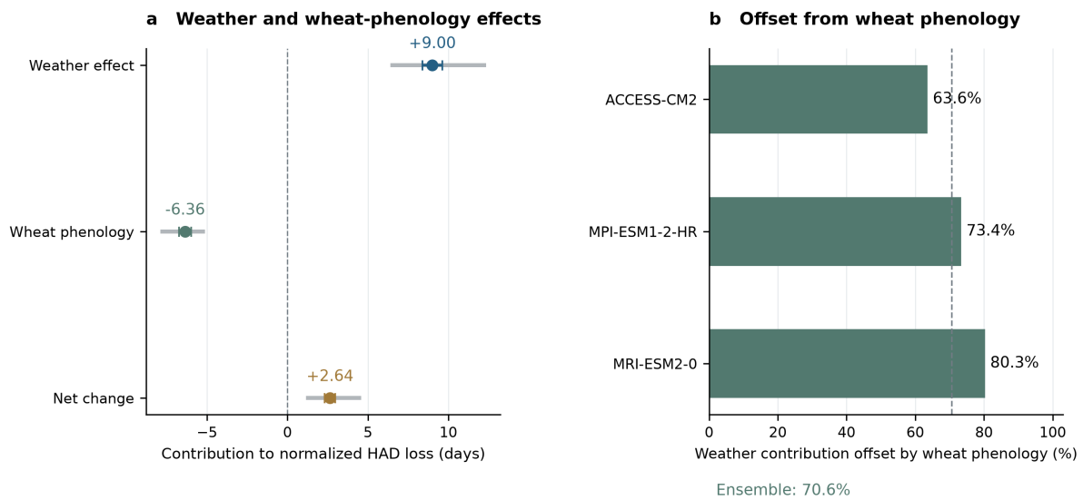
Figure 4 | Wheat phenology offsets part of the weather contribution to Septoria damage. (a) Weather and wheat-phenology contributions to normalized HAD loss during grain filling, and their sum, under late-century SSP5-8.5. The phenology contribution includes changes in upper-leaf appearance and unfolding and the flowering-to-soft-dough interval. The analysis uses 64 harvested-area-proportional draws at 62 cells and 5,731 valid season pairs. Grey segments span climate-model means; coloured whiskers show one spatial Monte Carlo standard error. Each Shapley contribution includes half of the weather-phenology interaction, shown separately in Supplementary Fig. S16. (b) Percentage of the weather contribution offset by wheat phenology in each climate model. The dashed line shows the ratio of ensemble contributions, 70.6%. These comparisons separate effects within the model; they do not estimate the effectiveness of changing sowing dates or cultivars.
