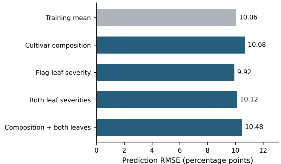
d Mixture-held-out predictions, 2019
