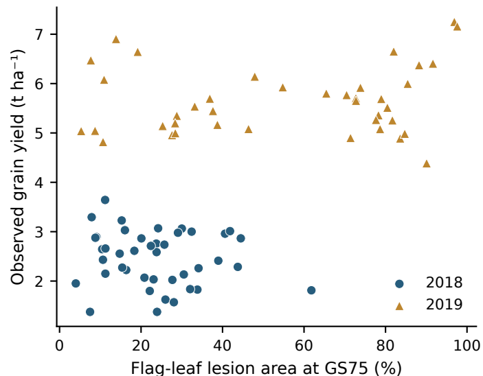
a Leaf damage and annual yield differences
