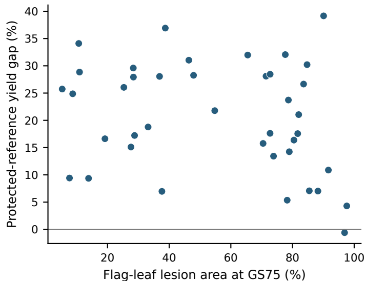
c Management-associated yield gaps, 2019
