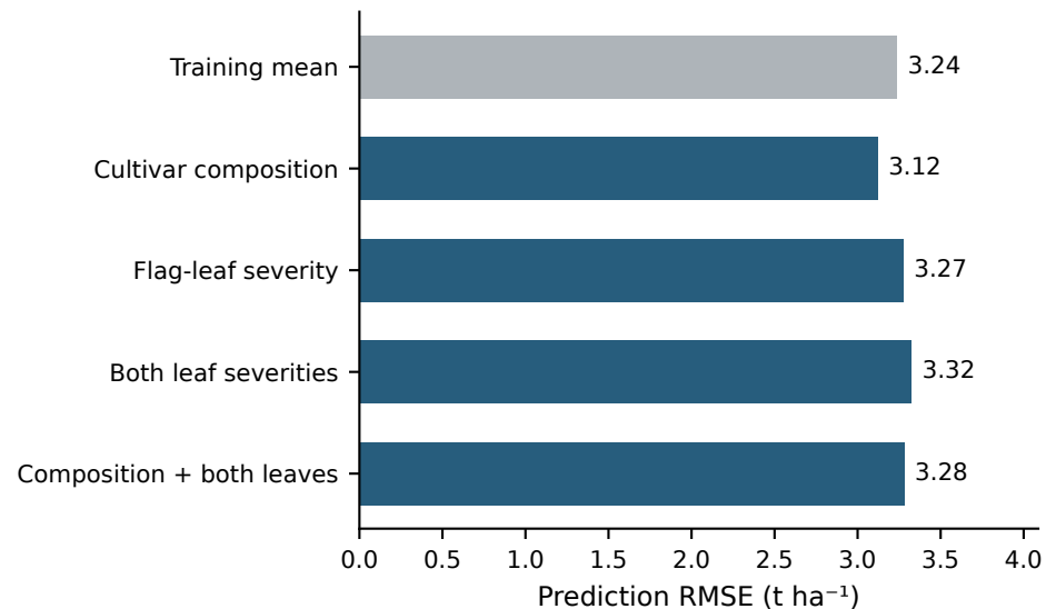
b Transfer between 2018 and 2019
