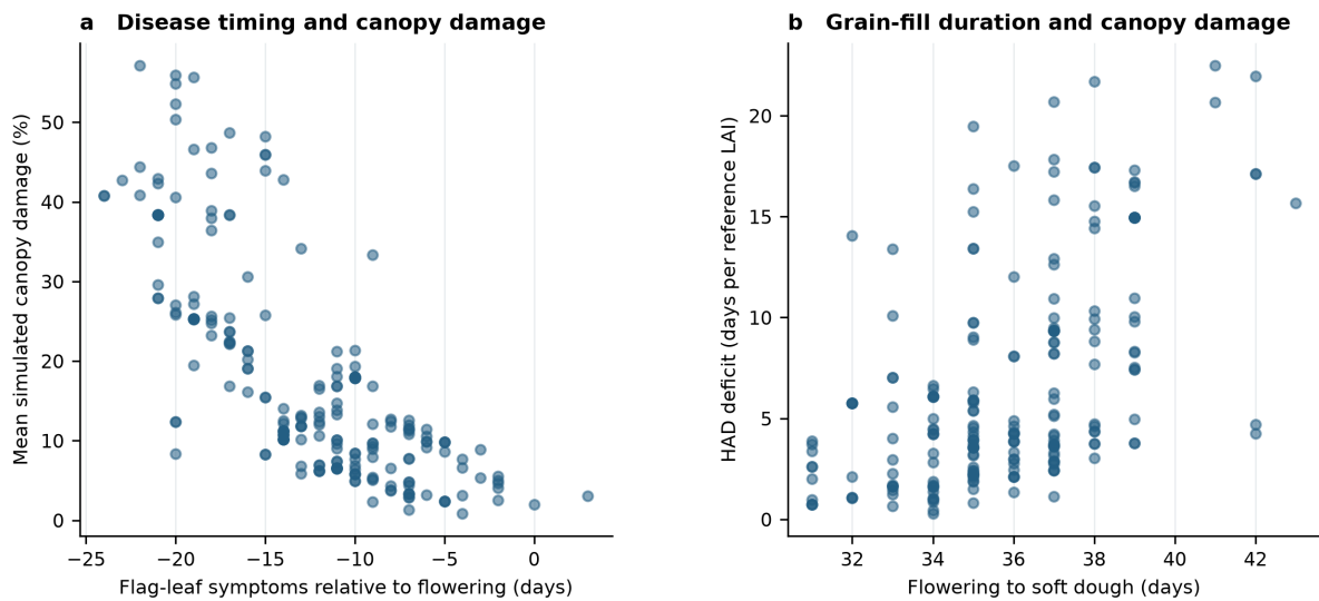
Figure S8 | Simulated disease timing and grain-fill duration in field weather replays. Each point represents one of 218 full-season simulations. (a) Flag-leaf symptoms relative to flowering and reference-area-weighted functional-canopy loss. (b) Flowering-to-soft-dough duration and HAD deficit. Reference upper-three-leaf LAI is nominally one. Both axes describe simulated quantities; these relationships do not validate observed disease severity or grain-yield loss.
