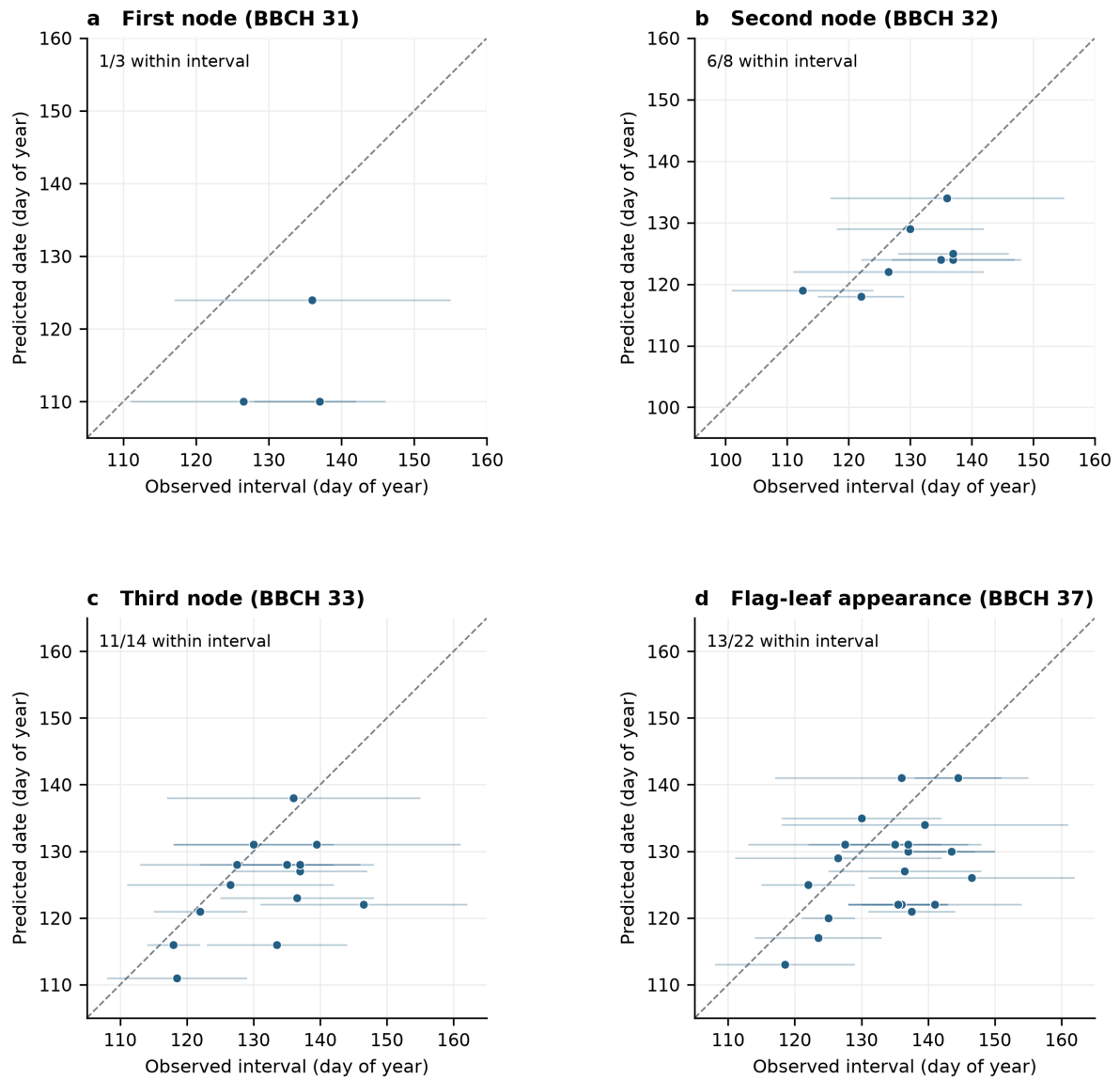
Figure S1 | Field evaluation of wheat development dates. Horizontal segments show observed two-sided stage intervals; their centers locate markers and are not treated as exact event dates. The dashed diagonal denotes equal dates, and an interval intersecting it contains the prediction. Counts give compatible intervals among all informative records. Observations from both field archives are pooled; calibration and evaluation remain separate. Intervals express observation resolution rather than statistical confidence.
