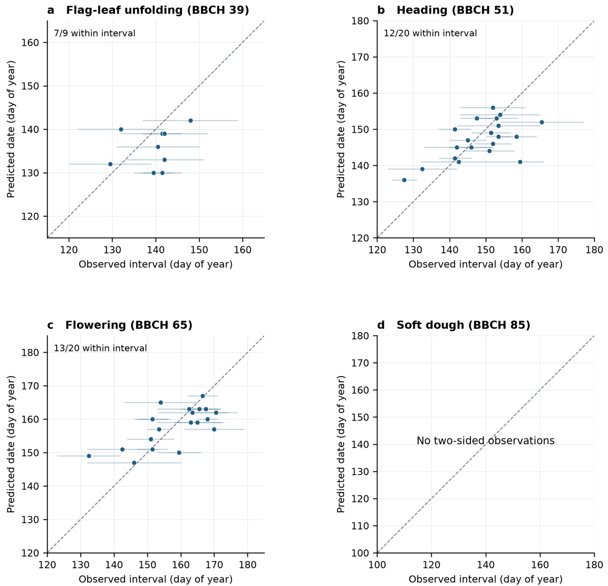
Figure S4 | Calibration of wheat development dates. Horizontal segments show observed two-sided stage intervals; their centers locate markers and are not treated as exact event dates. The dashed diagonal denotes equal dates, and an interval intersecting it contains the prediction. Counts give compatible intervals among all informative records. Observations from both field archives are pooled; calibration and evaluation remain separate. Intervals express observation resolution rather than statistical confidence.
