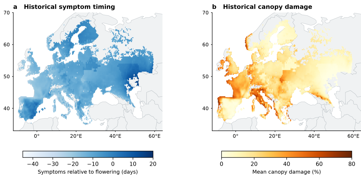
Figure S14 | Historical simulated disease timing and canopy damage across the full wheat domain. Panels show the 1991-2020 reference means on the corresponding valid late-century SSP5-8.5 paired support, averaged across three climate models. (a) Flag-leaf symptoms relative to flowering. (b) Grain-fill reference-area-weighted functional-canopy loss. Gray wheat pixels have unavailable estimates. These modeled reference distributions differ from observed historical disease prevalence.
