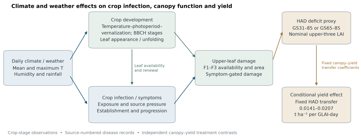
Figure S17 | Climate-crop-infection pathways linking canopy damage to conditional yield effects. Daily temperature, humidity and rainfall drive the retained crop-development and disease-weather operators. Development determines modeled leaf availability, unfolding and renewal, while weather and fixed source assumptions drive infection and symptom progression. Symptom-gated upper-three-leaf damage is integrated against a nominal reference canopy over GS31-85 or GS65-85 to give the healthy-area-duration (HAD) deficit proxy. Fixed coefficients of 0.0141-0.0207 t ha -1 per GLAI-day provide conditional yield-loss diagnostics. Crop-stage dates, source-numbered disease measurements and independent canopy-yield treatment contrasts constrain different links in the chain. The canopy reference, damage-to-functional-area conversion and current simulated yield effects have no local quantitative validation.
