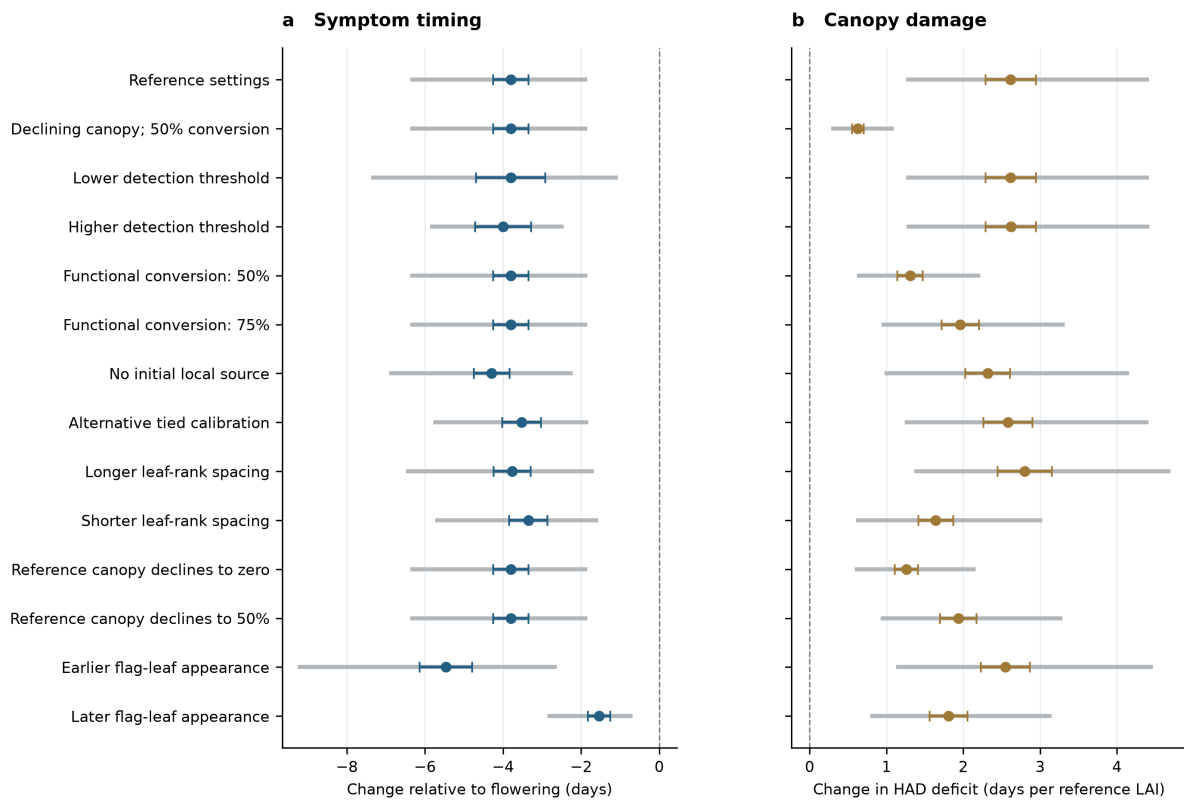
Figure S15 | Sensitivity of simulated climate responses to structural and reporting assumptions. (a) Flag-leaf symptom timing relative to flowering. (b) Grain-fill HAD deficit. All fourteen settings retain their common paired late-century SSP5–8.5 diagnostic population. Gray segments span three climate-model means; colored whiskers show one spatial Monte Carlo standard error for 64 area-proportional draws. Settings describe selected model assumptions rather than a probability distribution of future disease outcomes; precise settings and coverage remain in Supplementary Table S10.
