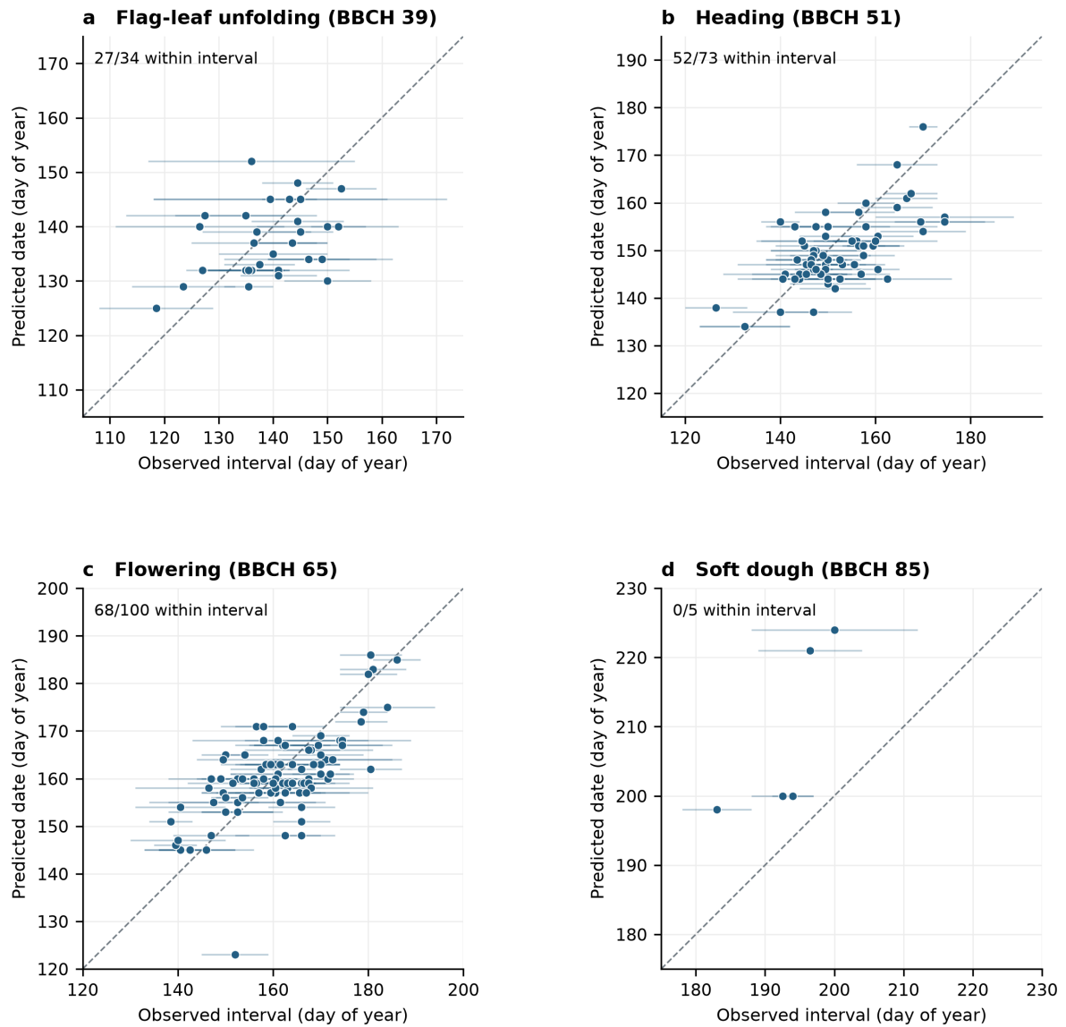
Figure S2 | Field evaluation of wheat development dates. Horizontal segments show observed two-sided stage intervals; their centers locate markers and are not treated as exact event dates. The dashed diagonal denotes equal dates, and an interval intersecting it contains the prediction. Counts give compatible intervals among all informative records. Observations from both field archives are pooled; calibration and evaluation remain separate. Intervals express observation resolution rather than statistical confidence.
