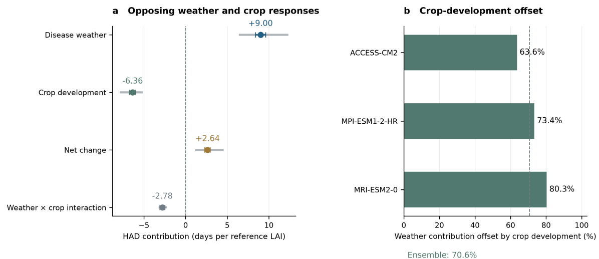
Figure S16 | Supported weather-crop decomposition and crop-development offsets. (a) Weather, crop-development and net HAD contributions with the full interaction shown separately. The interaction is already allocated equally between the two Shapley contributions and is not added again to the net. Gray segments span climate-model means; colored whiskers show one spatial Monte Carlo standard error. (b) Model-specific offsets and their ensemble-contribution ratio. The same 5,731 supported paired seasons underlie all HAD terms. These sampled diagnostic responses differ from full-grid impact estimates and do not measure intervention benefits.
