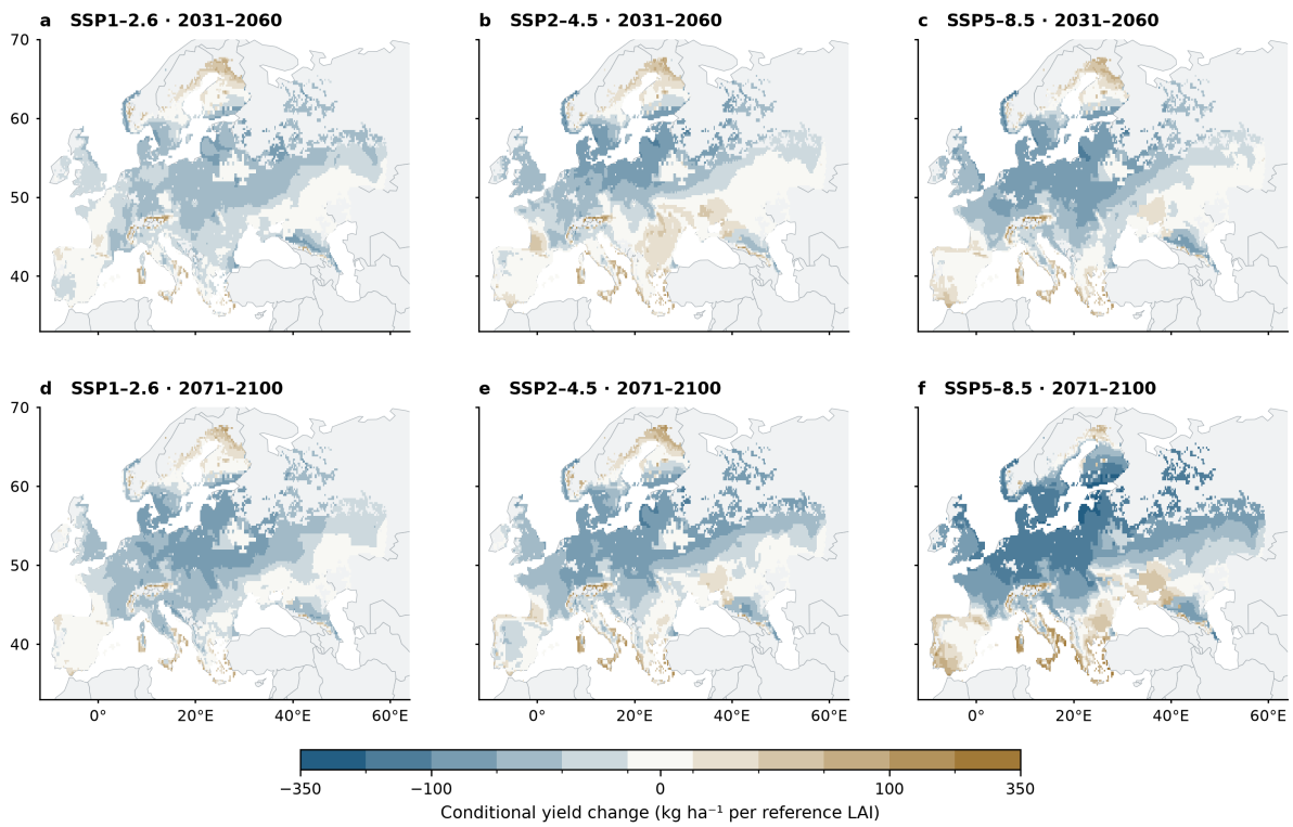
Figure S13 | Conditional disease-related yield changes. Panels show three-climate-model means at every eligible wheat land-use grid for two future periods relative to 1991–2020. Each figure shares symmetric discrete color intervals retaining the full data range. Gray wheat pixels have unavailable estimates. Timing requires detected symptoms in both paired years. Conditional yield change is -0.018 times the HAD-deficit change, converted to kg ha -1 per reference LAI. The yield product depends on a fixed canopy-yield coefficient and nominal leaf area rather than a validated grain-yield model.
