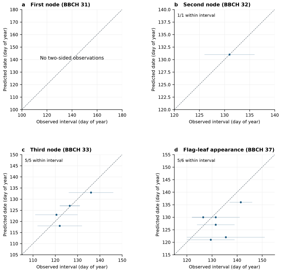
Figure S3 | Calibration of wheat development dates. Horizontal segments show observed two-sided stage intervals; their centers locate markers and are not treated as exact event dates. The dashed diagonal denotes equal dates, and an interval intersecting it contains the prediction. Counts give compatible intervals among all informative records. Observations from both field archives are pooled; calibration and evaluation remain separate. Intervals express observation resolution rather than statistical confidence.
