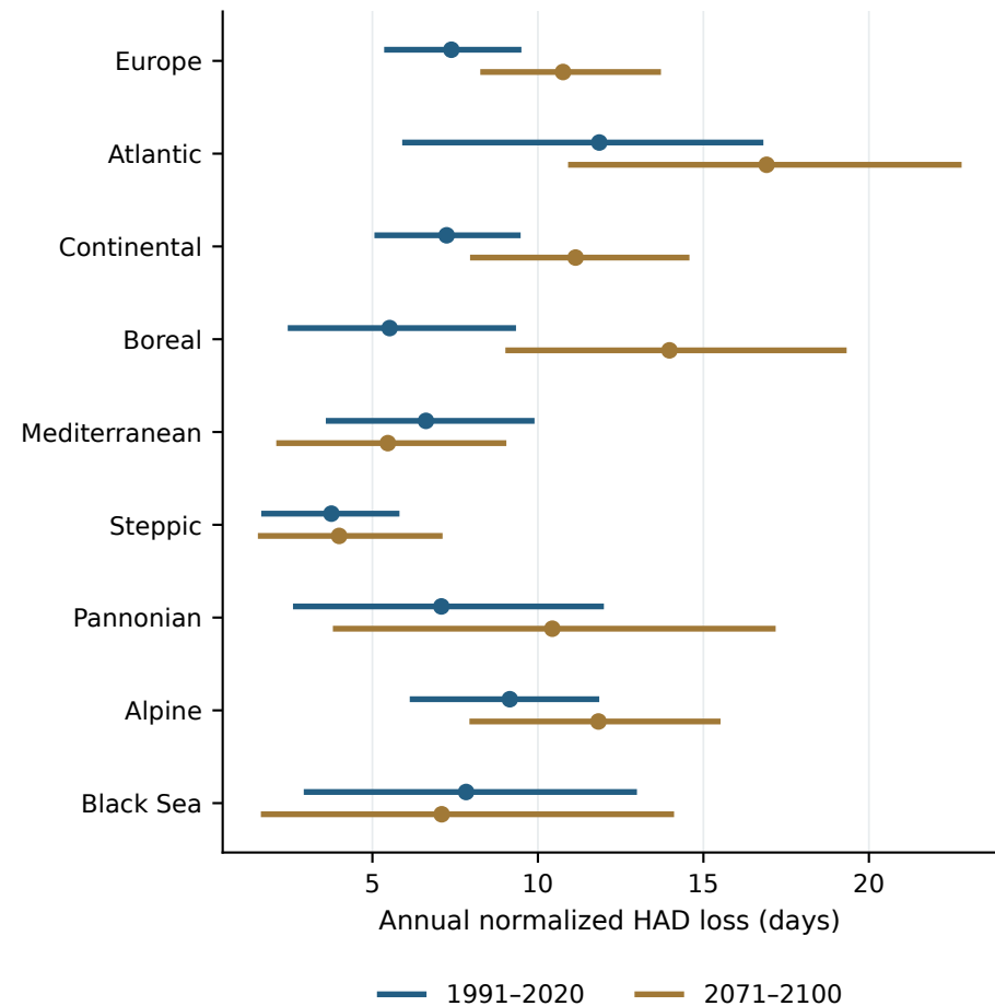
a Annual mean and 10th-90th quantiles
