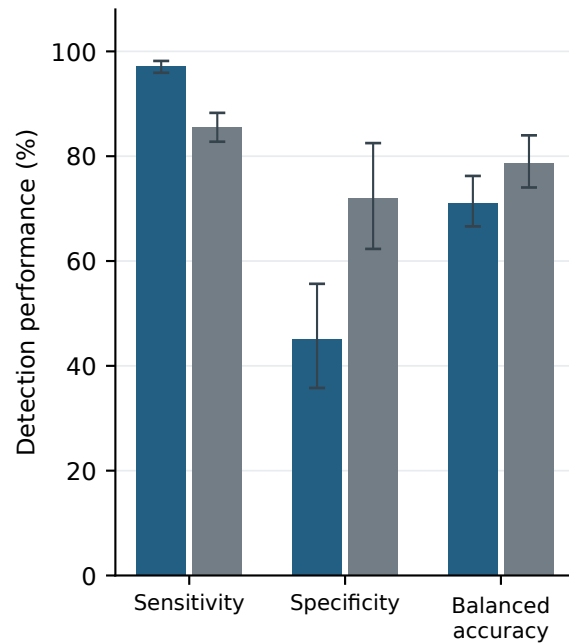
c Symptom detection
