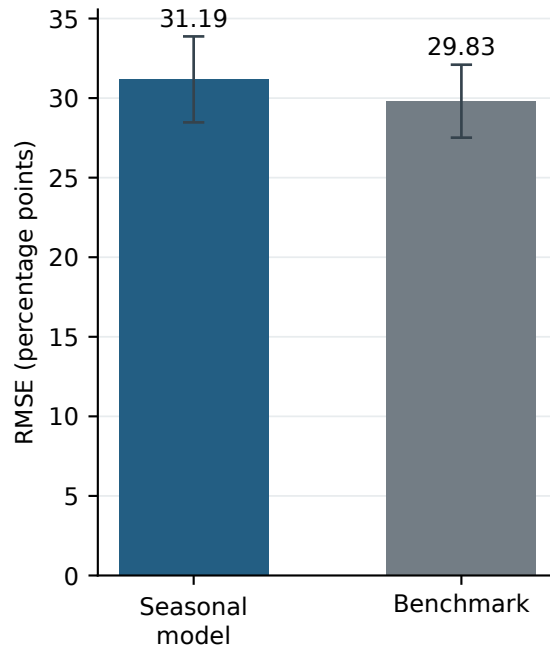
b Severity prediction error
