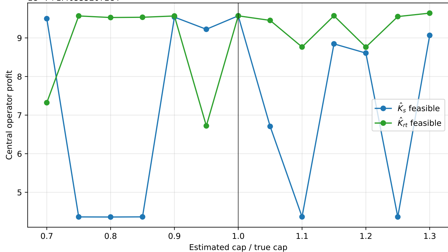
Figure 4.a: Effect of Ks/Krt Estimation Error on Operator Profit
