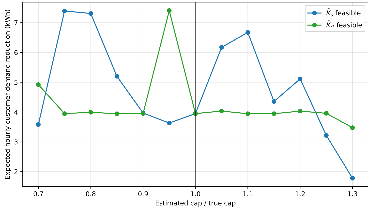
Figure 4.b: Effect of Ks/Krt Estimation Error on Customer DR
