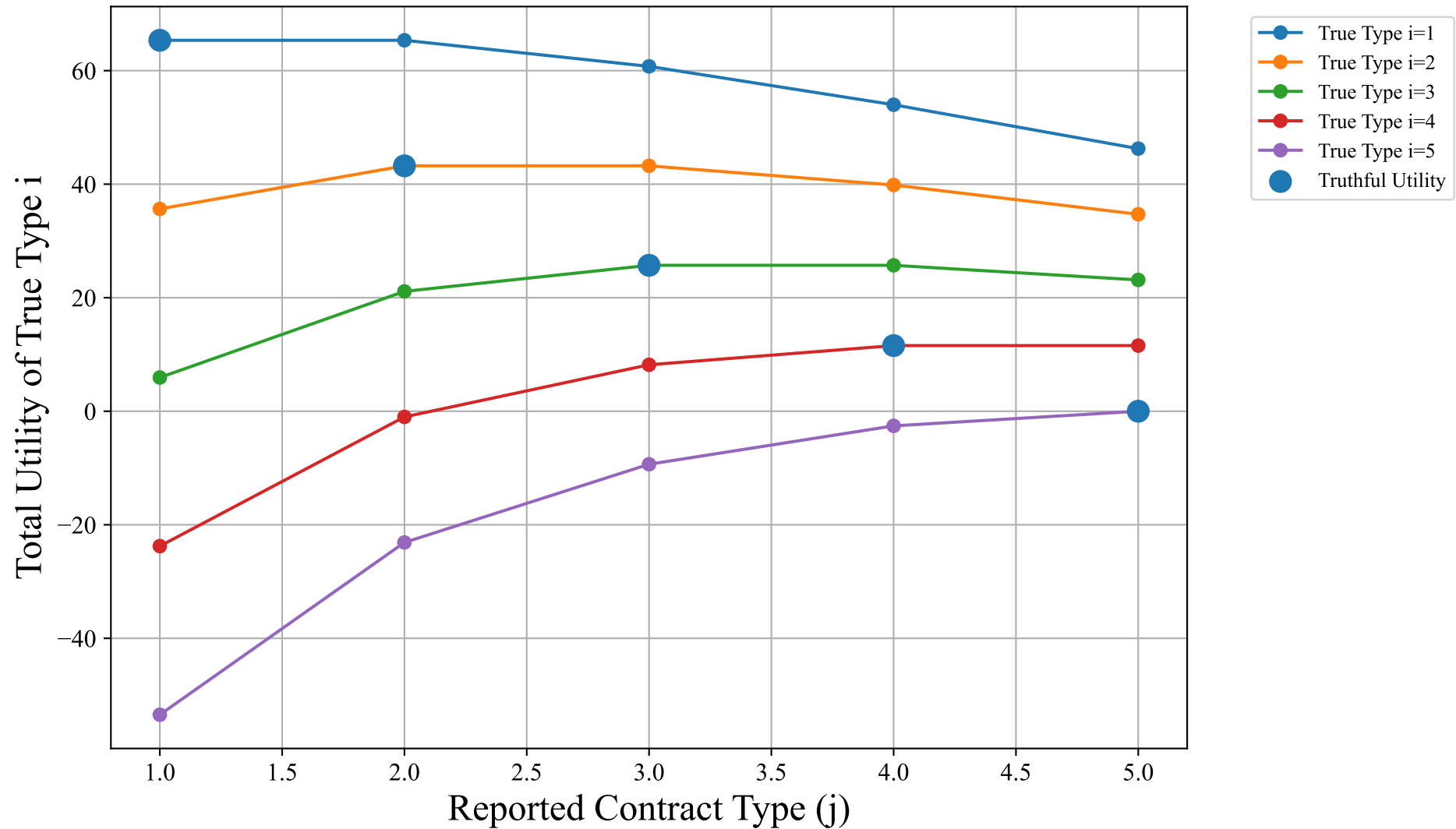
Robust Proposed Contract: IC Check, r=0.1
