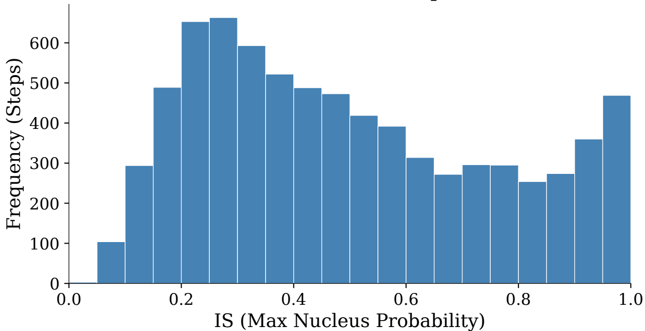
IS Distribution (GSM, Epoch 16)
