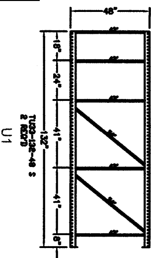
11' x 48" 14 Gauge Pigeon Hole Upright w/Built- In Handrail Galvanized
