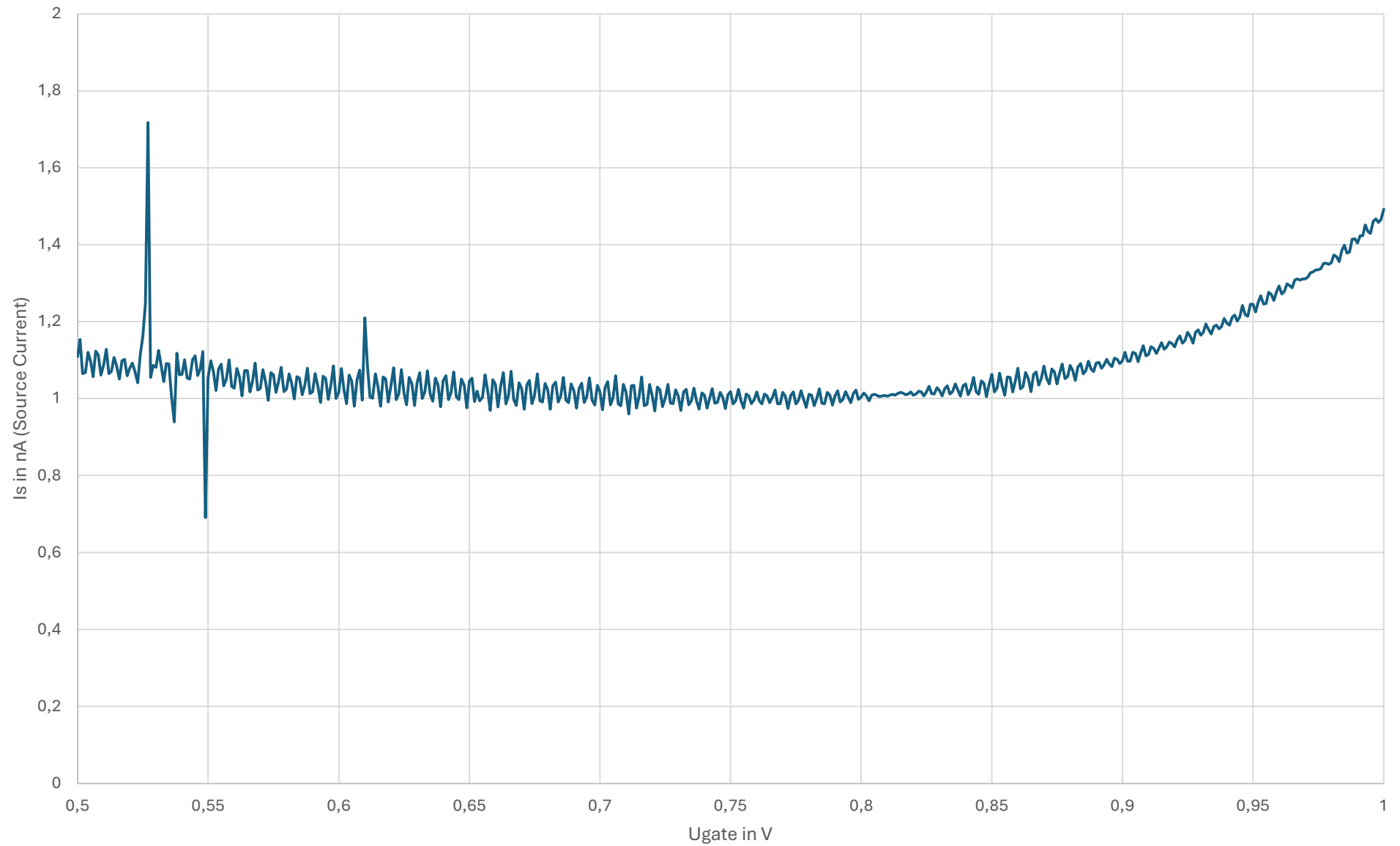
Source Current (device #01)
