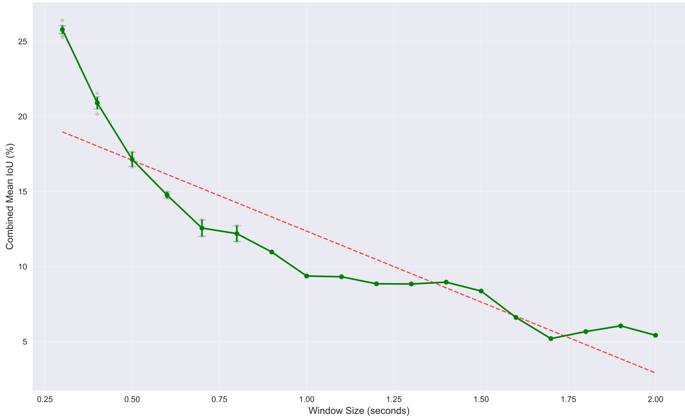
Combined Mean IoU Performance
