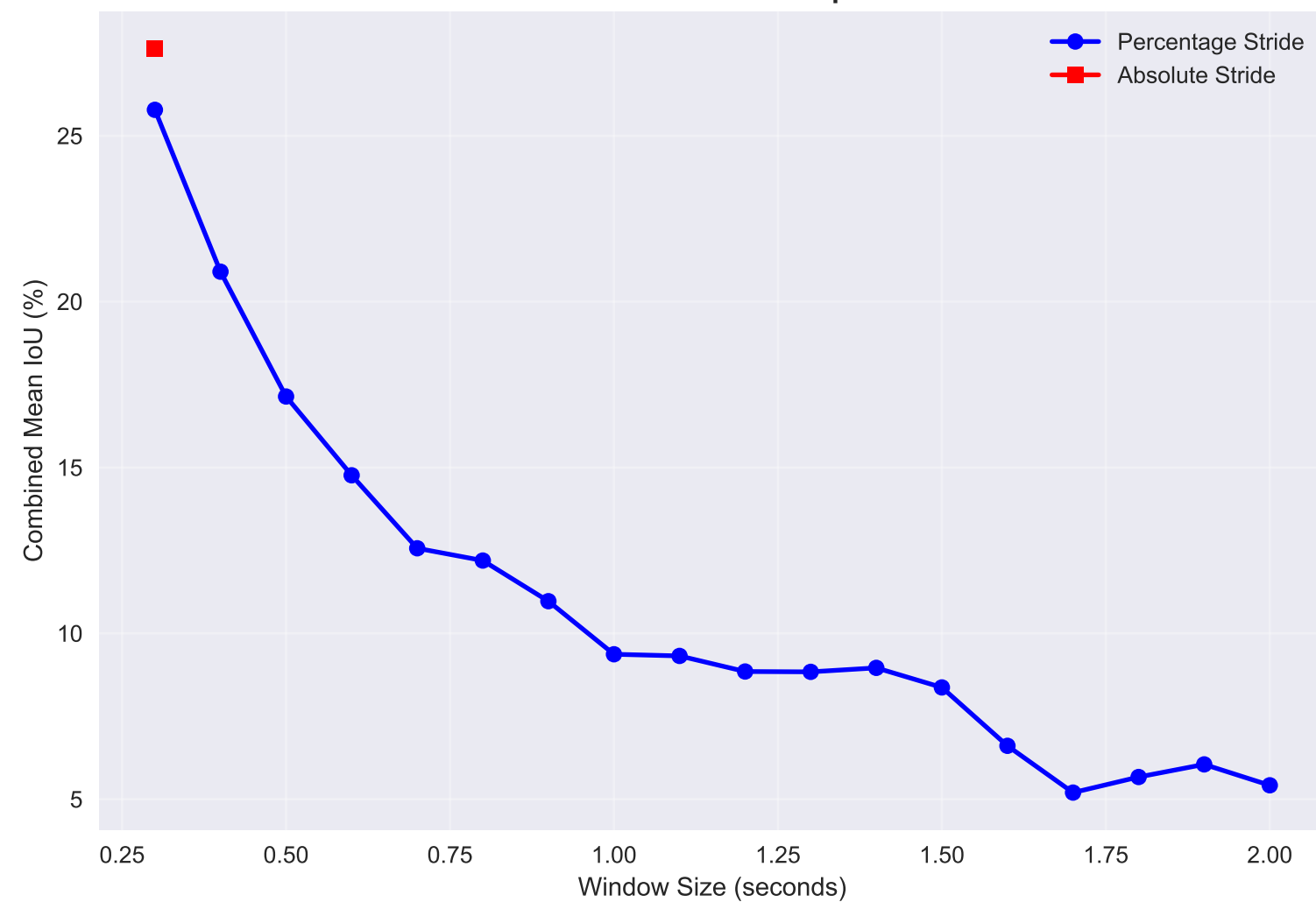
Combined Mean IoU Comparison
