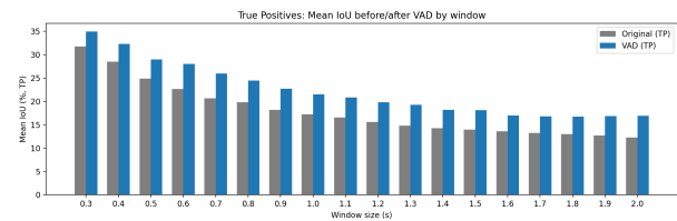
Fig. 8. Voice Activity Detection (VAD) IoU improvement results across different window
