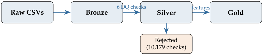
Figure 1: Bronze -> Silver -> Gold pipeline with rejected-records store.
