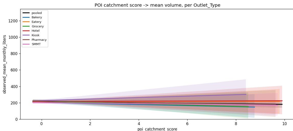
Figure 2: POI \times Outlet_Type interaction (notebook 23). Per-outlet POI counts have low absolute correlation with monthly volume regardless of channel, confirming POI’s role as a catchment signal rather than a direct predictor.
