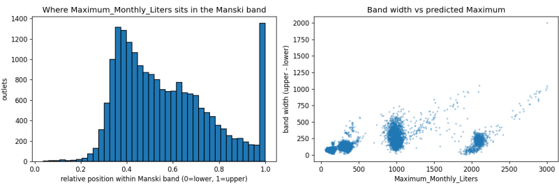
Figure 5: Per-outlet Manski band width. Band lower edge = \max(\text{lower\_bound}, \text{obs\_max}) ; upper edge = peer-q99 cap. Sensitivity sweep: across quantile \{0.85, 0.9, 0.95\} \times scheme \{\text{balanced, frontier-heavy, plateau-heavy}\} \times cap multiplier \{2..6\} , median uplift stays at 1.250\times and cap-binding at 0 %.
