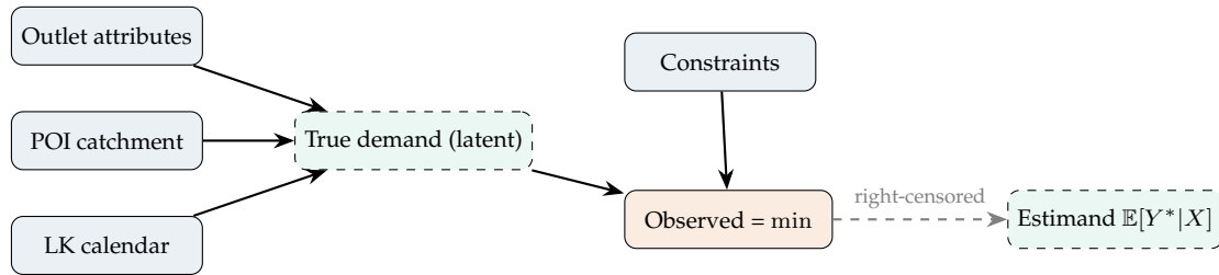
Figure 3: DAG. Solid arrows are observed; dashed arrow indicates partial identification of the estimand from \min(\cdot) .
