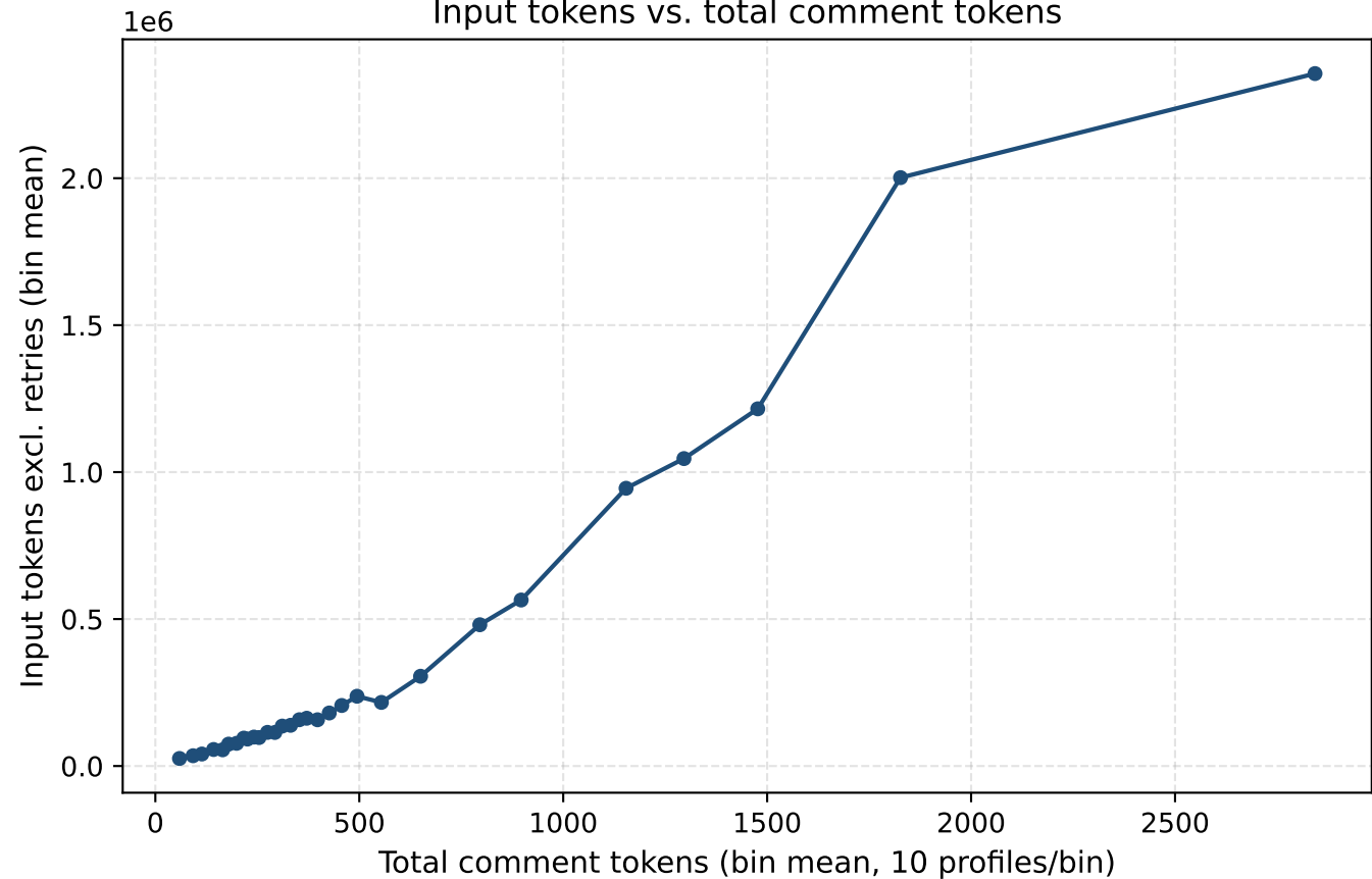
Input tokens vs. total comment tokens
